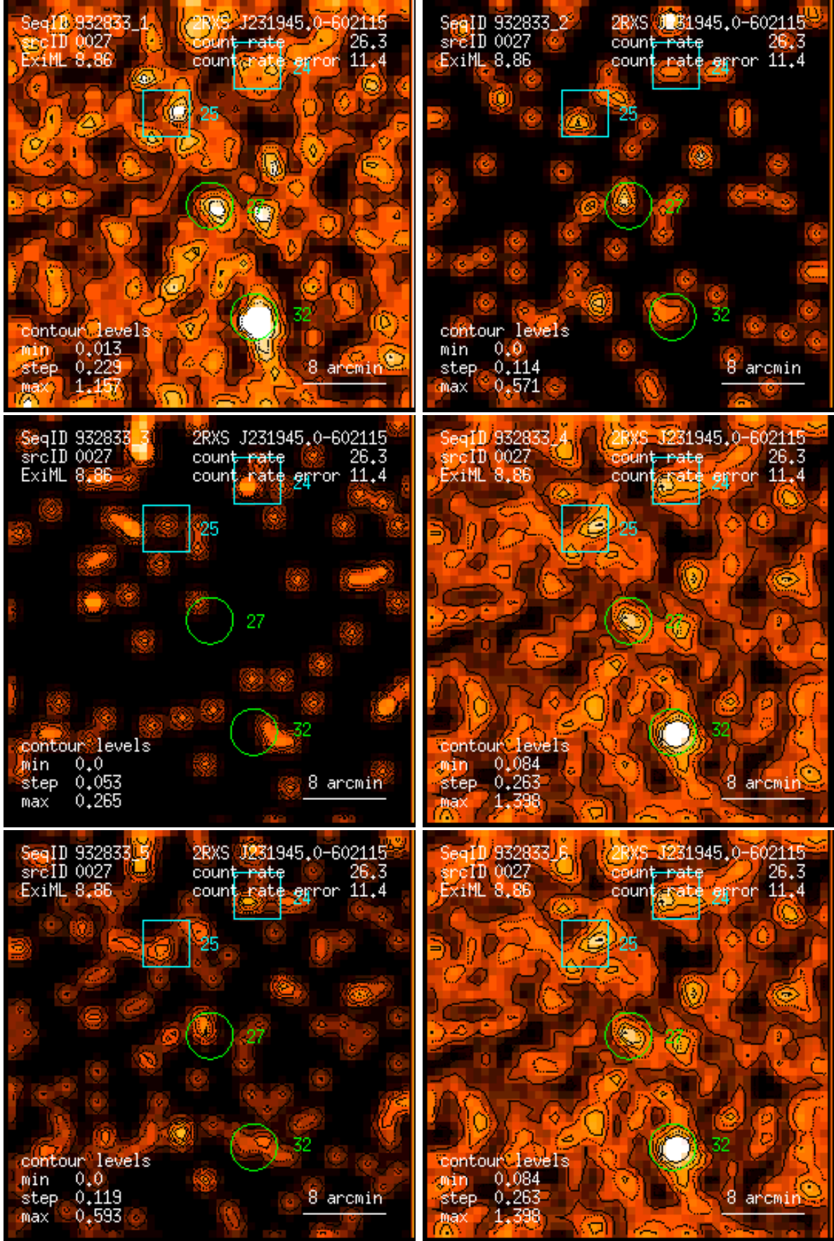
Figure 27: RASS 932833: detection 0027: band rate images, Gaussian filter: (1) PSPC channels 11 – 41, (2) 52 – 90, (3) 91 – 201, (4) 11 – 235, (5) 52 – 201, (6) 11 – 201. Broad band rates in counts/ks. Band rate contour levels in counts/ks/arcmin 2 .
