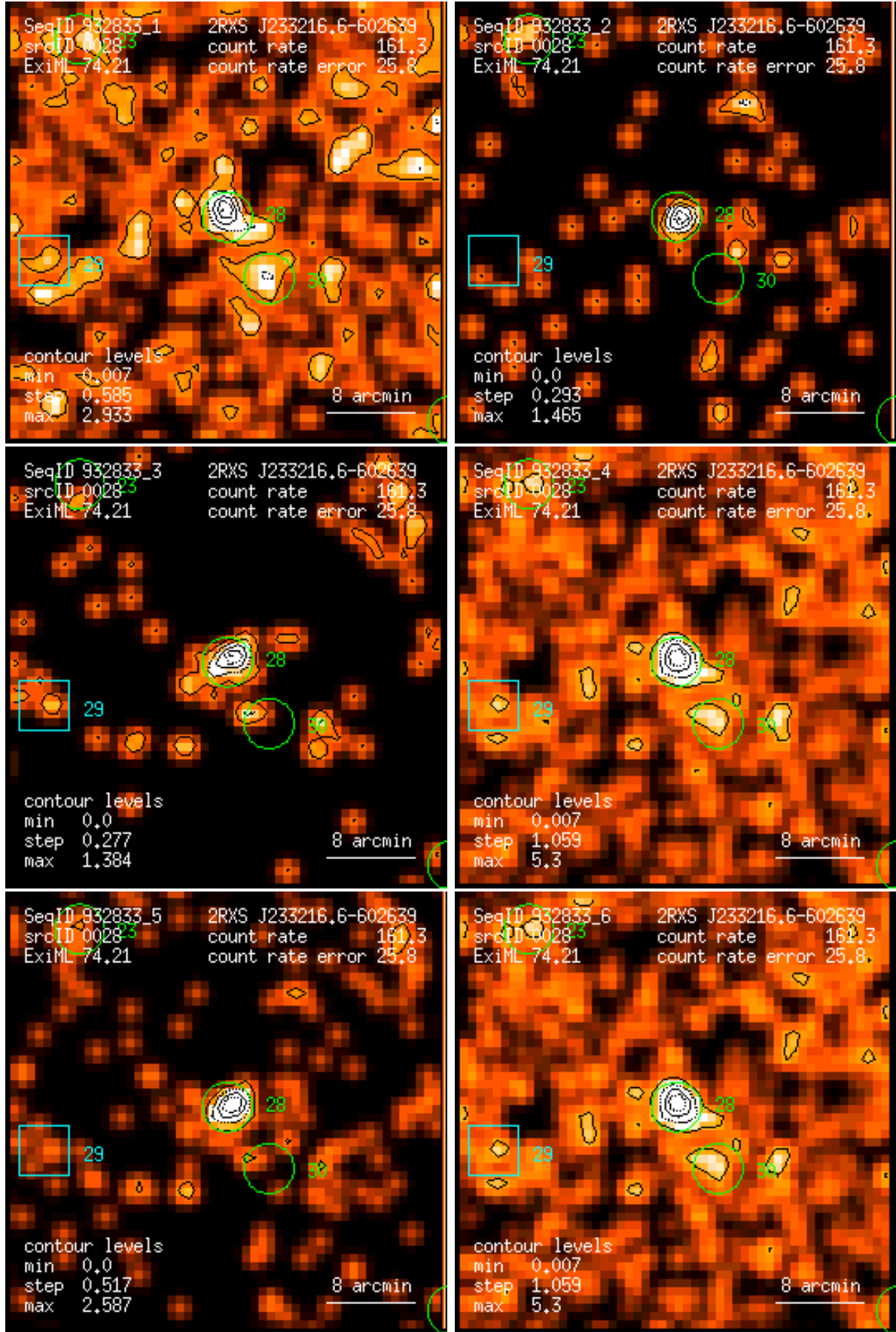
Figure 28: RASS 932833: detection 0028: band rate images, Gaussian filter: (1) PSPC channels 11 – 41, (2) 52 – 90, (3) 91 – 201, (4) 11 – 235, (5) 52 – 201, (6) 11 – 201. Broad band rates in counts/ks. Band rate contour levels in counts/ks/arcmin 2 .
