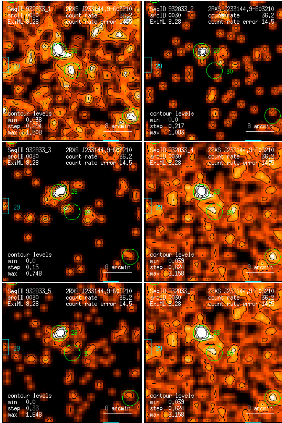
Figure 30: RASS 932833: detection 0030: band rate images, Gaussian filter: (1) PSPC channels 11 – 41, (2) 52 – 90, (3) 91 – 201, (4) 11 – 235, (5) 52 – 201, (6) 11 – 201. Broad band rates in counts/ks. Band rate contour levels in counts/ks/arcmin 2 .
