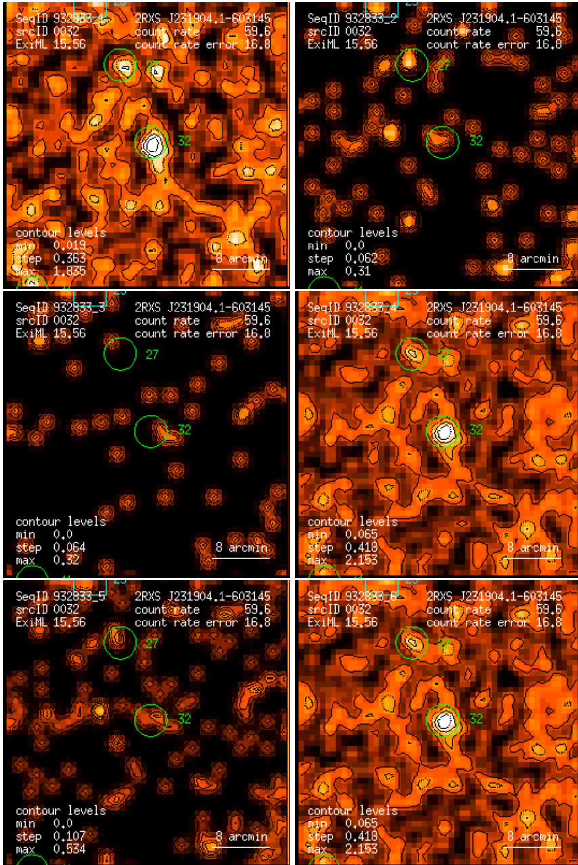
Figure 32: RASS 932833: detection 0032: band rate images, Gaussian filter: (1) PSPC channels 11 – 41, (2) 52 – 90, (3) 91 – 201, (4) 11 – 235, (5) 52 – 201, (6) 11 – 201. Broad band rates in counts/ks. Band rate contour levels in counts/ks/arcmin 2 .
