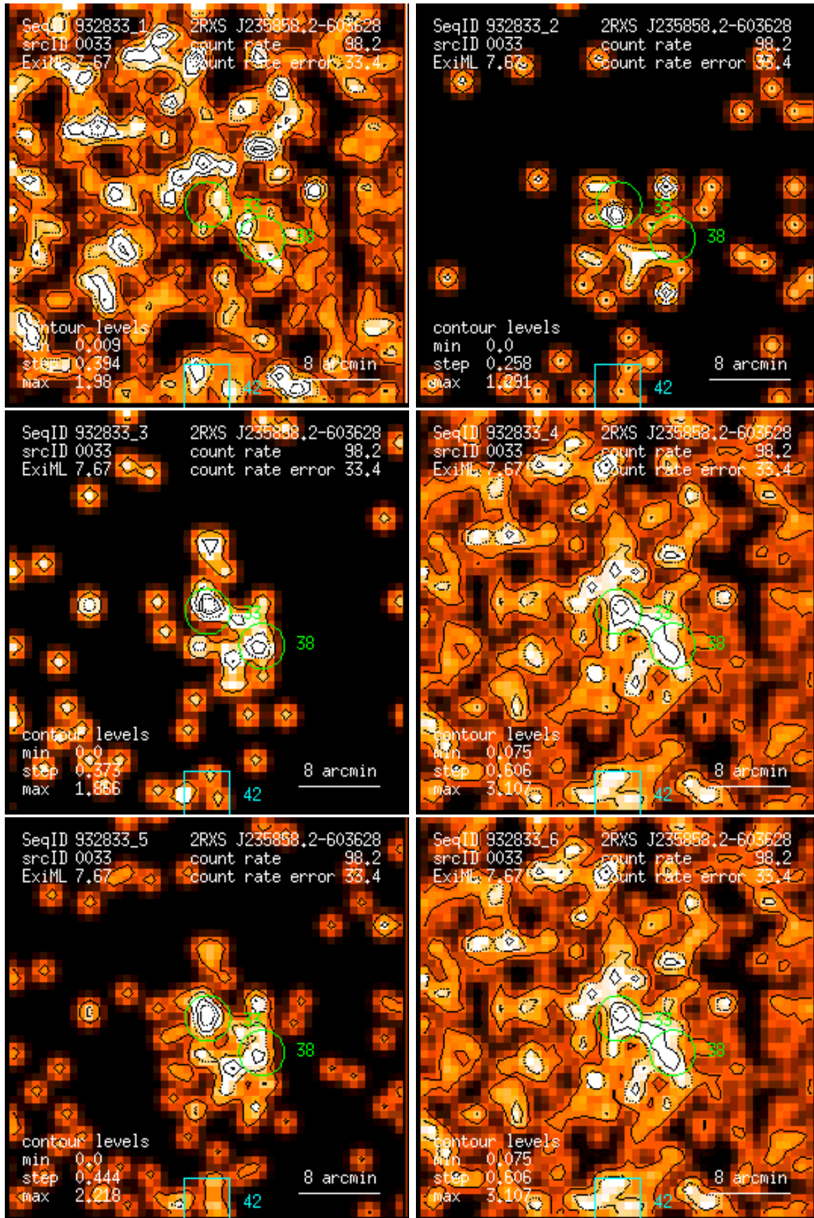
Figure 33: RASS 932833: detection 0033: band rate images, Gaussian filter: (1) PSPC channels 11 – 41, (2) 52 – 90, (3) 91 – 201, (4) 11 – 235, (5) 52 – 201, (6) 11 – 201. Broad band rates in counts/ks. Band rate contour levels in counts/ks/arcmin 2 .
