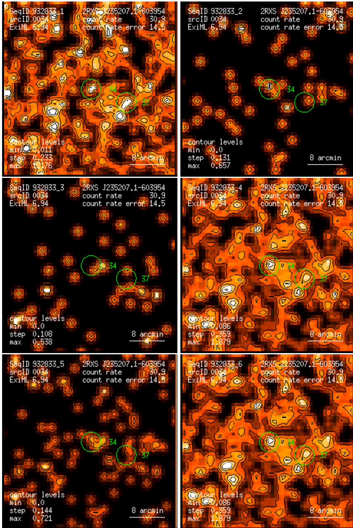
Figure 34: RASS 932833: detection 0034: band rate images, Gaussian filter: (1) PSPC channels 11 – 41, (2) 52 – 90, (3) 91 – 201, (4) 11 – 235, (5) 52 – 201, (6) 11 – 201. Broad band rates in counts/ks. Band rate contour levels in counts/ks/arcmin 2 .
