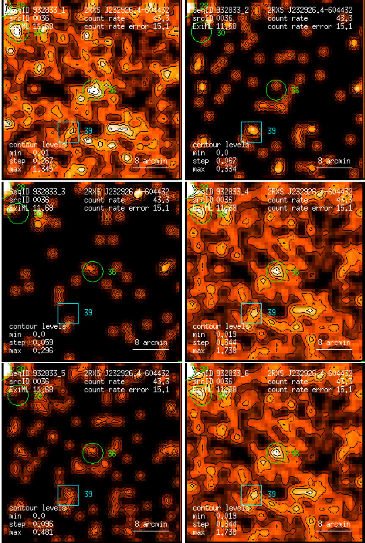
Figure 36: RASS 932833: detection 0036: band rate images, Gaussian filter: (1) PSPC channels 11 – 41, (2) 52 – 90, (3) 91 – 201, (4) 11 – 235, (5) 52 – 201, (6) 11 – 201. Broad band rates in counts/ks. Band rate contour levels in counts/ks/arcmin 2 .
