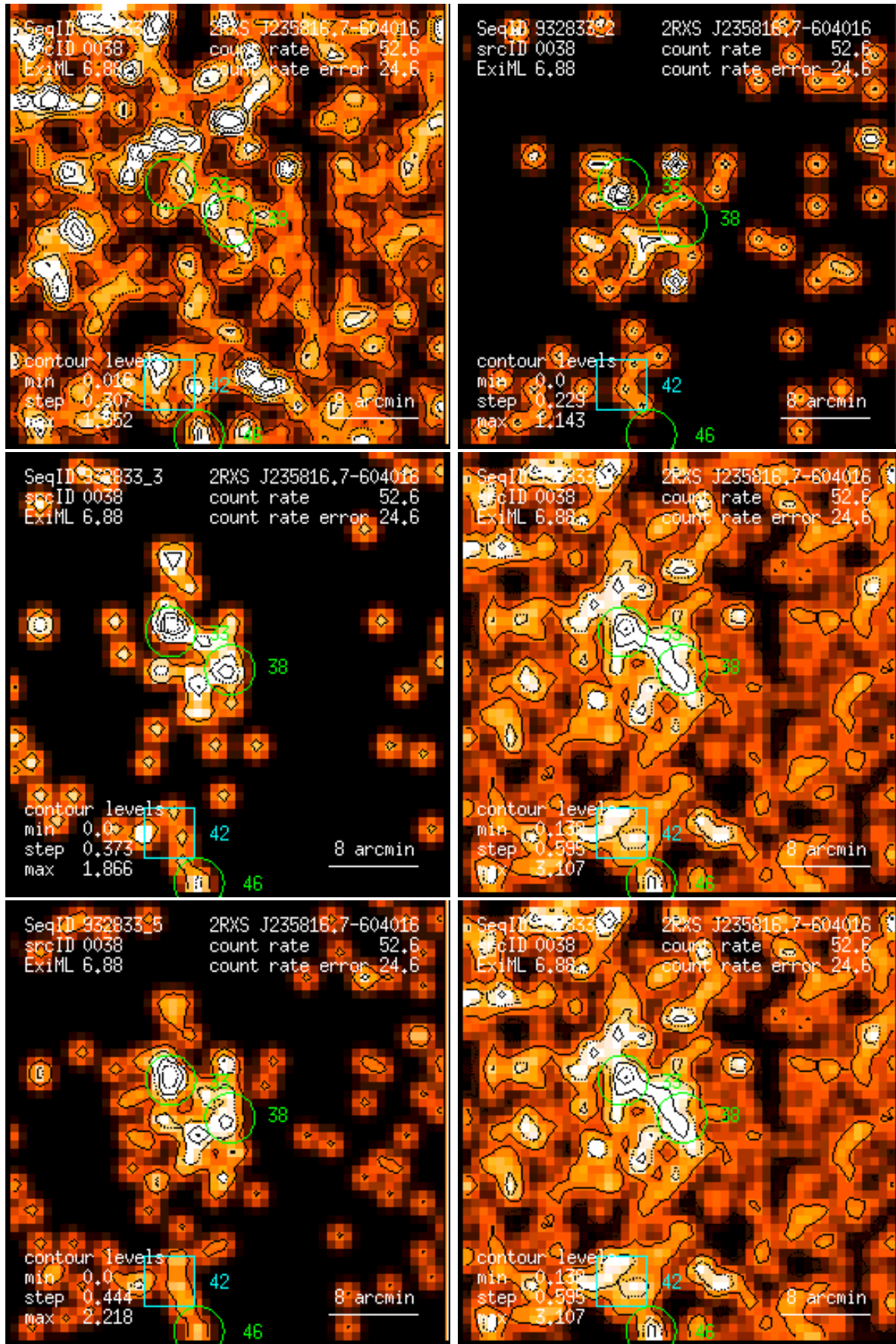
Figure 38: RASS 932833: detection 0038: band rate images, Gaussian filter: (1) PSPC channels 11 – 41, (2) 52 – 90, (3) 91 – 201, (4) 11 – 235, (5) 52 – 201, (6) 11 – 201. Broad band rates in counts/ks. Band rate contour levels in counts/ks/arcmin 2 .
