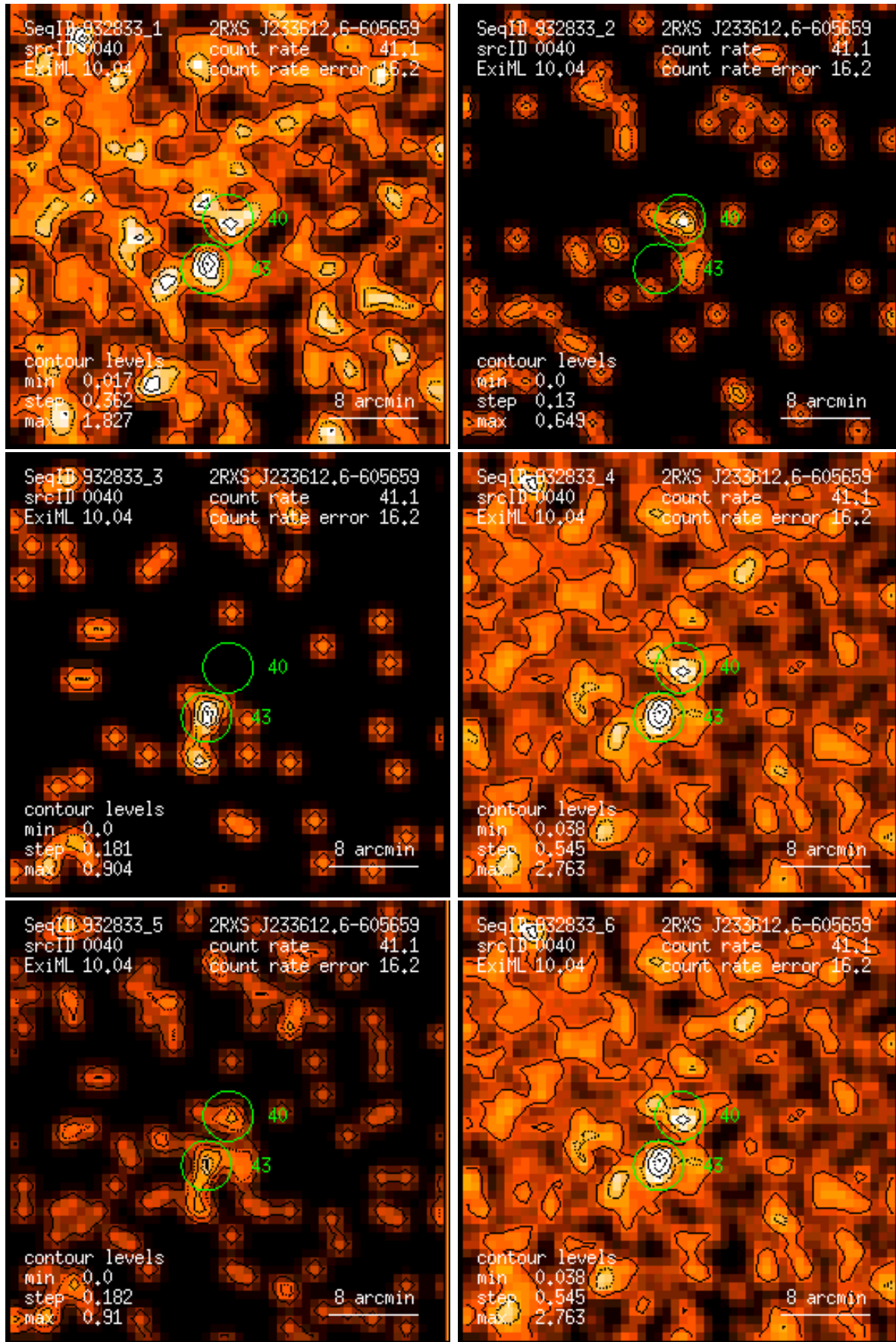
Figure 40: RASS 932833: detection 0040: band rate images, Gaussian filter: (1) PSPC channels 11 – 41, (2) 52 – 90, (3) 91 – 201, (4) 11 – 235, (5) 52 – 201, (6) 11 – 201. Broad band rates in counts/ks. Band rate contour levels in counts/ks/arcmin 2 .
