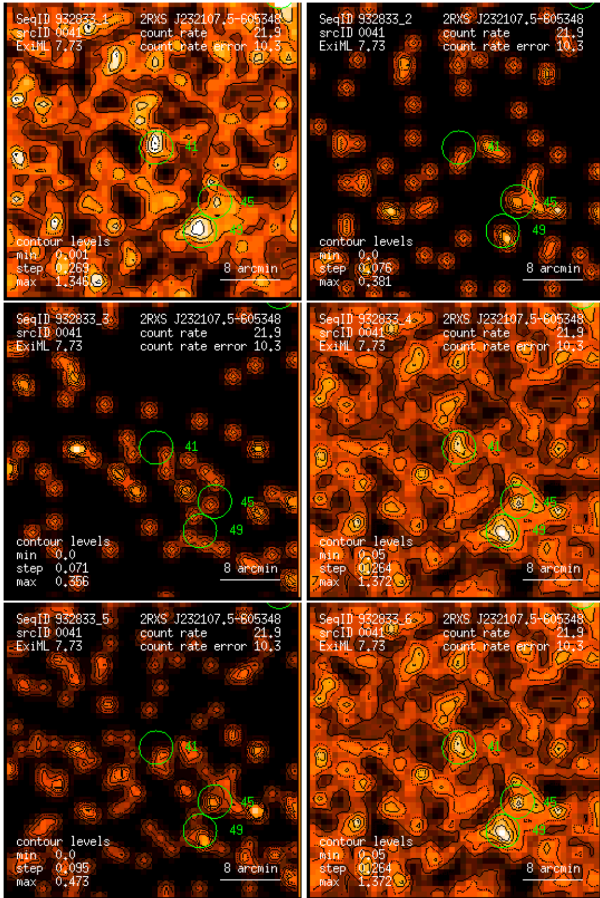
Figure 41: RASS 932833: detection 0041: band rate images, Gaussian filter: (1) PSPC channels 11 – 41, (2) 52 – 90, (3) 91 – 201, (4) 11 – 235, (5) 52 – 201, (6) 11 – 201. Broad band rates in counts/ks. Band rate contour levels in counts/ks/arcmin 2 .
