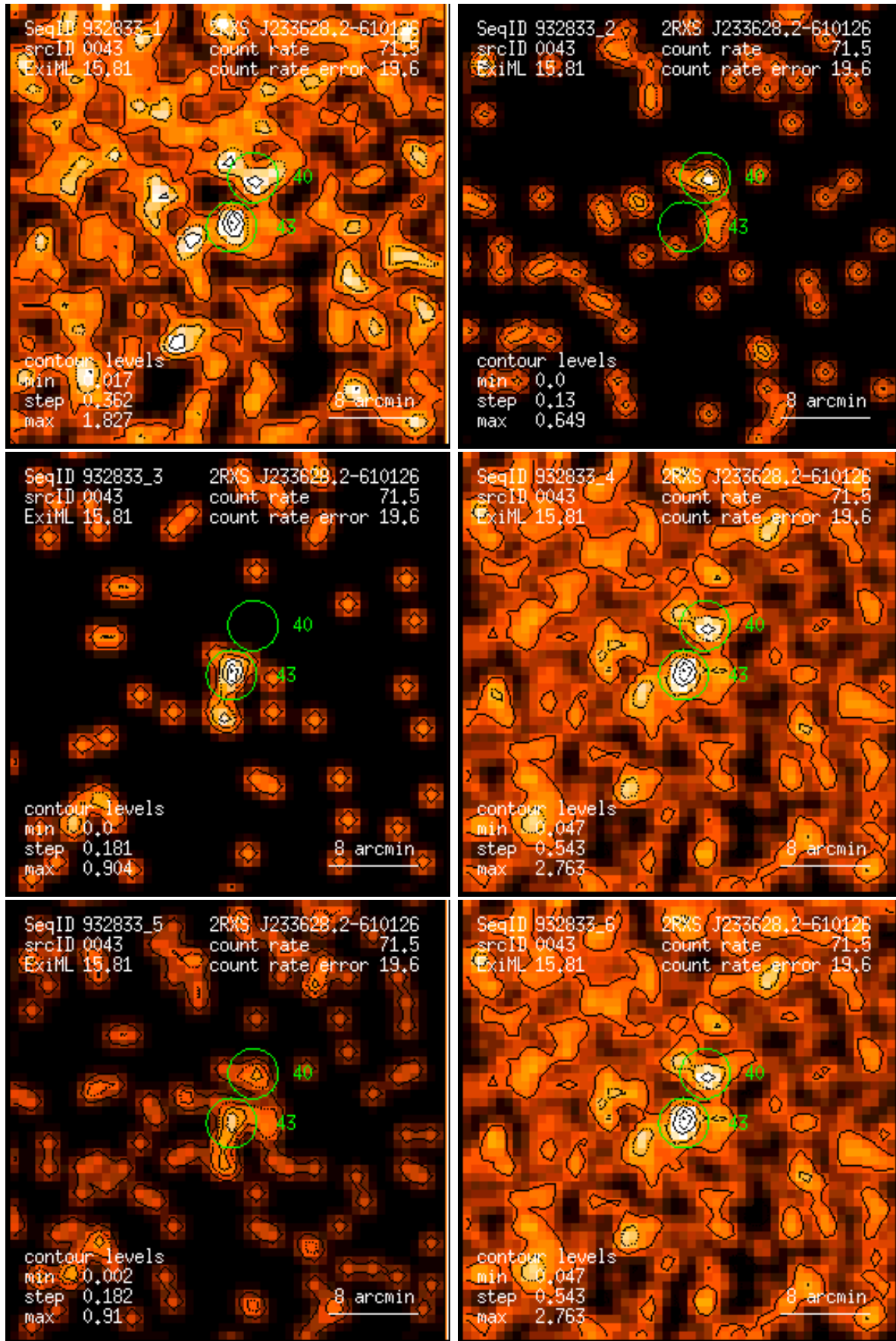
Figure 43: RASS 932833: detection 0043: band rate images, Gaussian filter: (1) PSPC channels 11 – 41, (2) 52 – 90, (3) 91 – 201, (4) 11 – 235, (5) 52 – 201, (6) 11 – 201. Broad band rates in counts/ks. Band rate contour levels in counts/ks/arcmin 2 .
