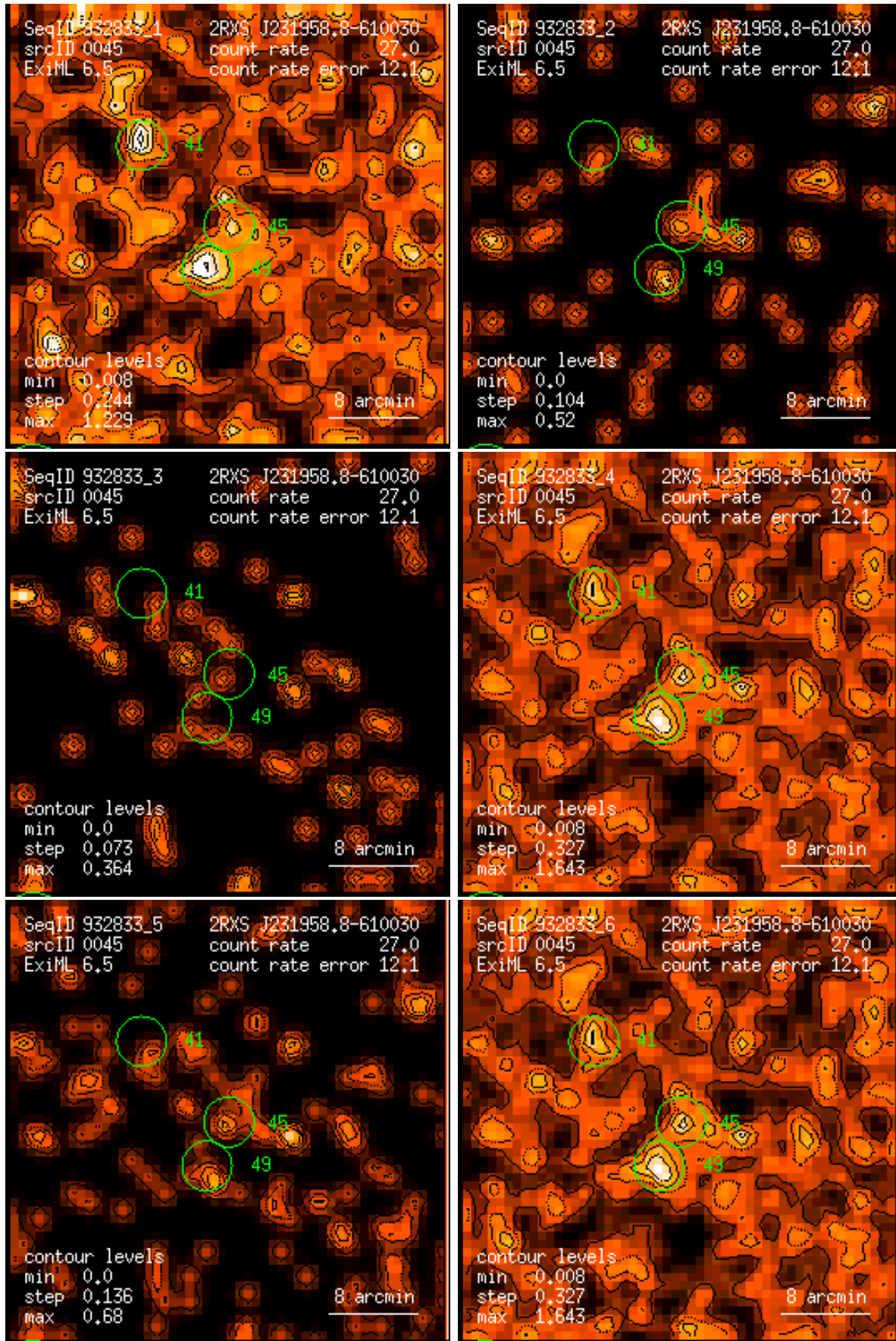
Figure 45: RASS 932833: detection 0045: band rate images, Gaussian filter: (1) PSPC channels 11 – 41, (2) 52 – 90, (3) 91 – 201, (4) 11 – 235, (5) 52 – 201, (6) 11 – 201. Broad band rates in counts/ks. Band rate contour levels in counts/ks/arcmin 2 .
