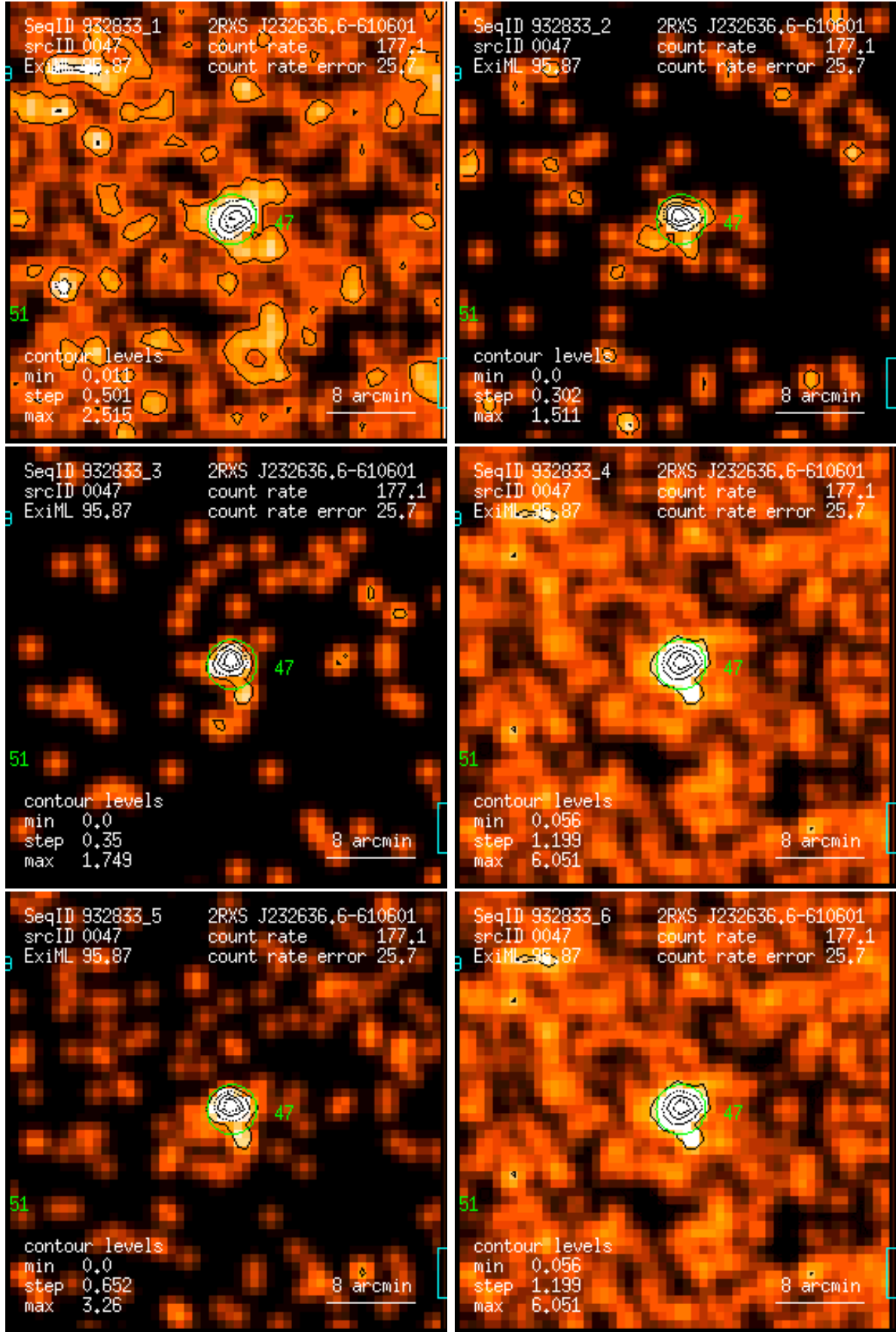
Figure 47: RASS 932833: detection 0047: band rate images, Gaussian filter: (1) PSPC channels 11 – 41, (2) 52 – 90, (3) 91 – 201, (4) 11 – 235, (5) 52 – 201, (6) 11 – 201. Broad band rates in counts/ks. Band rate contour levels in counts/ks/arcmin 2 .
