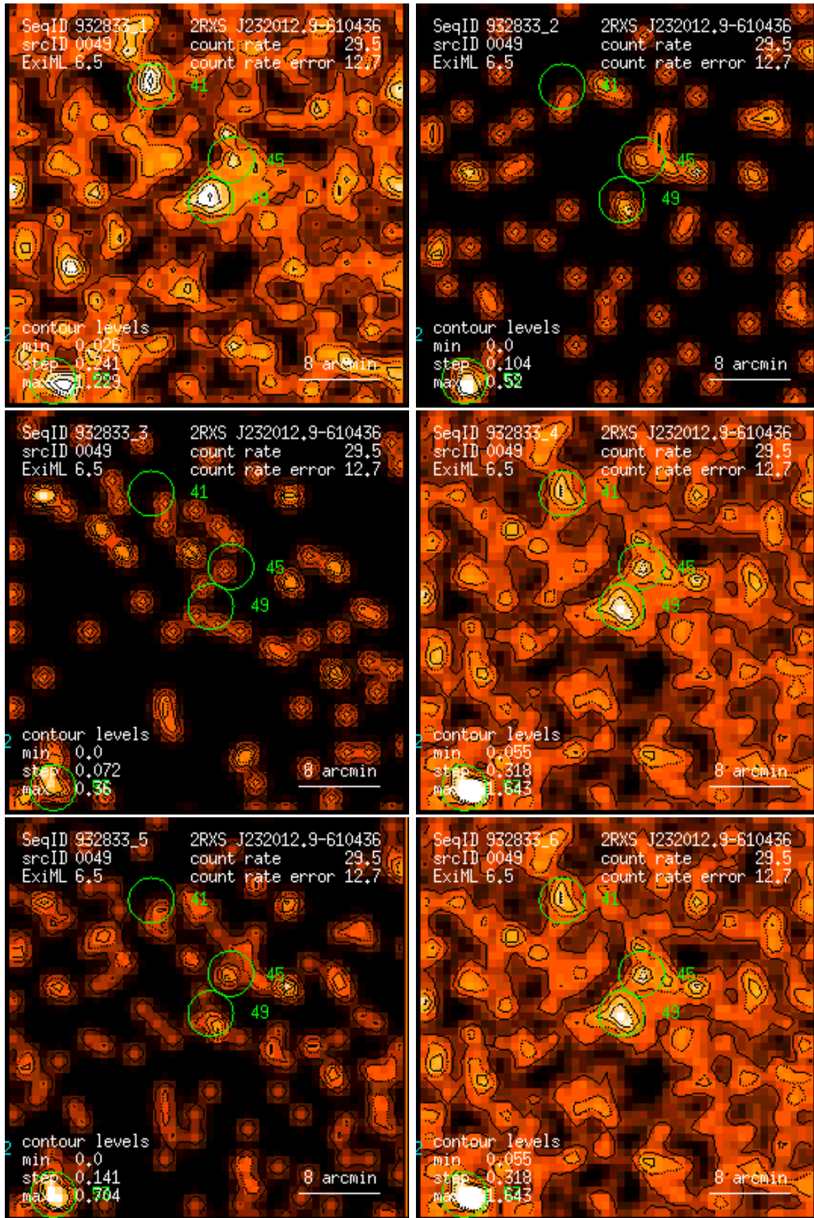
Figure 49: RASS 932833: detection 0049: band rate images, Gaussian filter: (1) PSPC channels 11 – 41, (2) 52 – 90, (3) 91 – 201, (4) 11 – 235, (5) 52 – 201, (6) 11 – 201. Broad band rates in counts/ks. Band rate contour levels in counts/ks/arcmin 2 .
