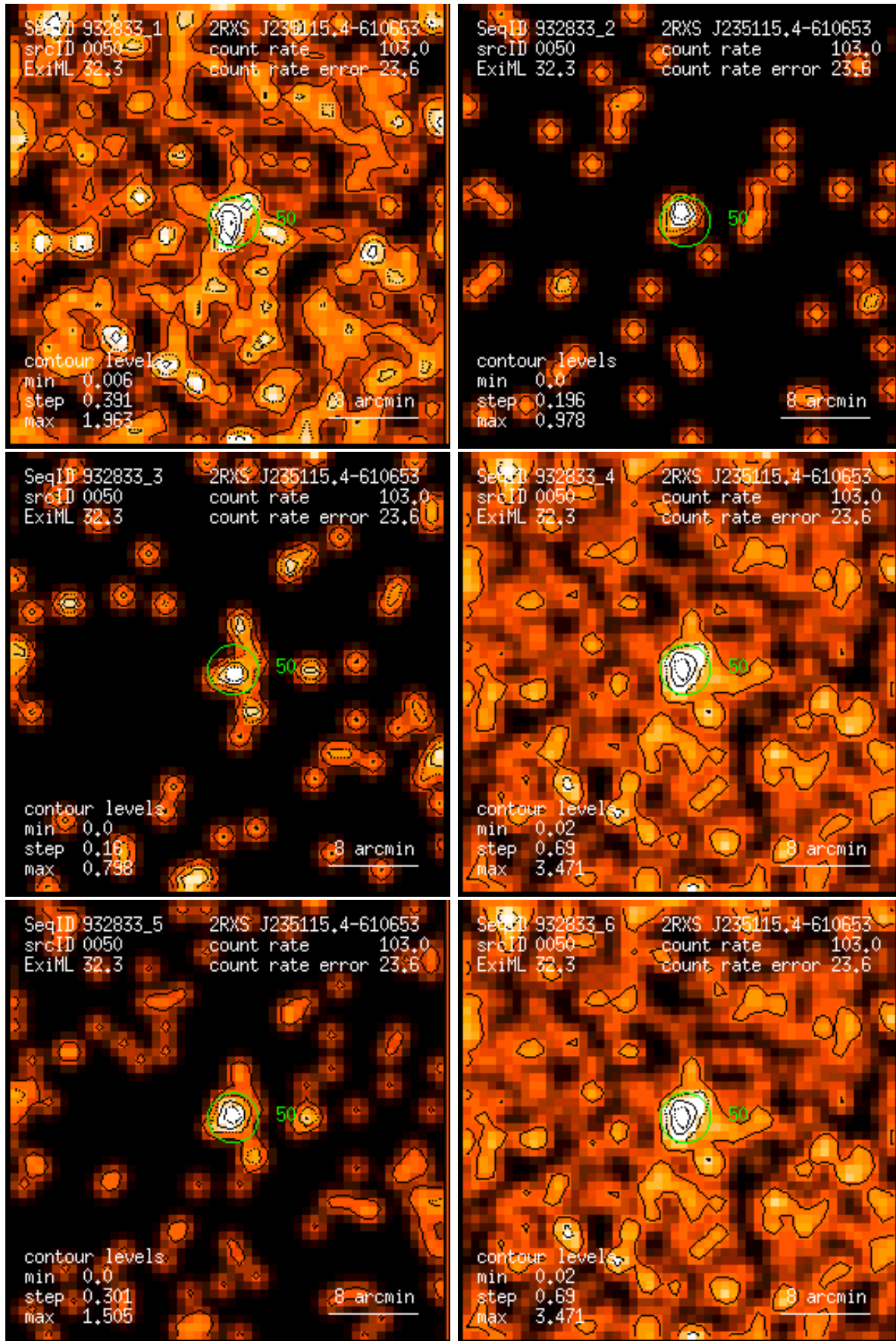
Figure 50: RASS 932833: detection 0050: band rate images, Gaussian filter: (1) PSPC channels 11 – 41, (2) 52 – 90, (3) 91 – 201, (4) 11 – 235, (5) 52 – 201, (6) 11 – 201. Broad band rates in counts/ks. Band rate contour levels in counts/ks/arcmin 2 .
