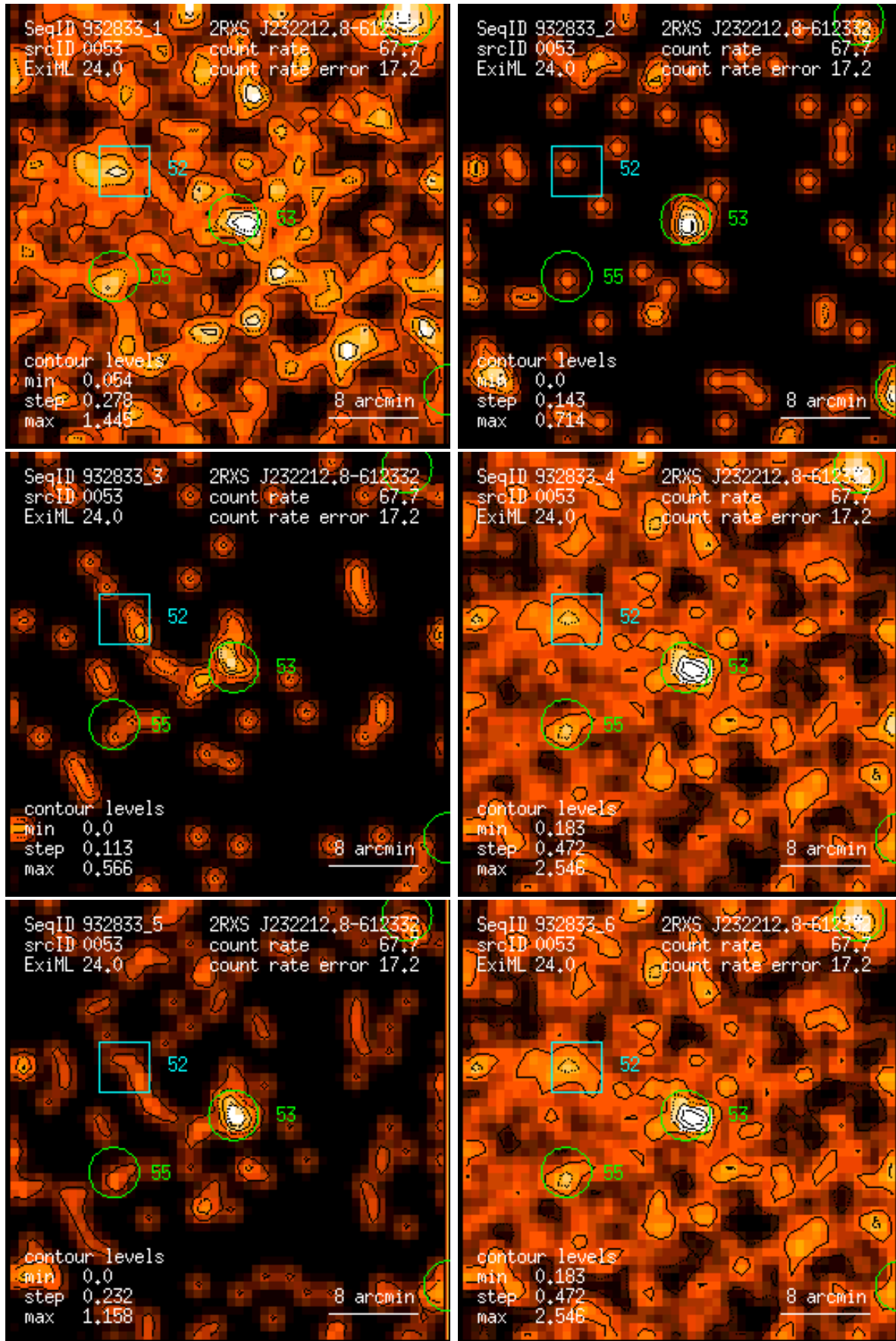
Figure 53: RASS 932833: detection 0053: band rate images, Gaussian filter: (1) PSPC channels 11 – 41, (2) 52 – 90, (3) 91 – 201, (4) 11 – 235, (5) 52 – 201, (6) 11 – 201. Broad band rates in counts/ks. Band rate contour levels in counts/ks/arcmin 2 .
