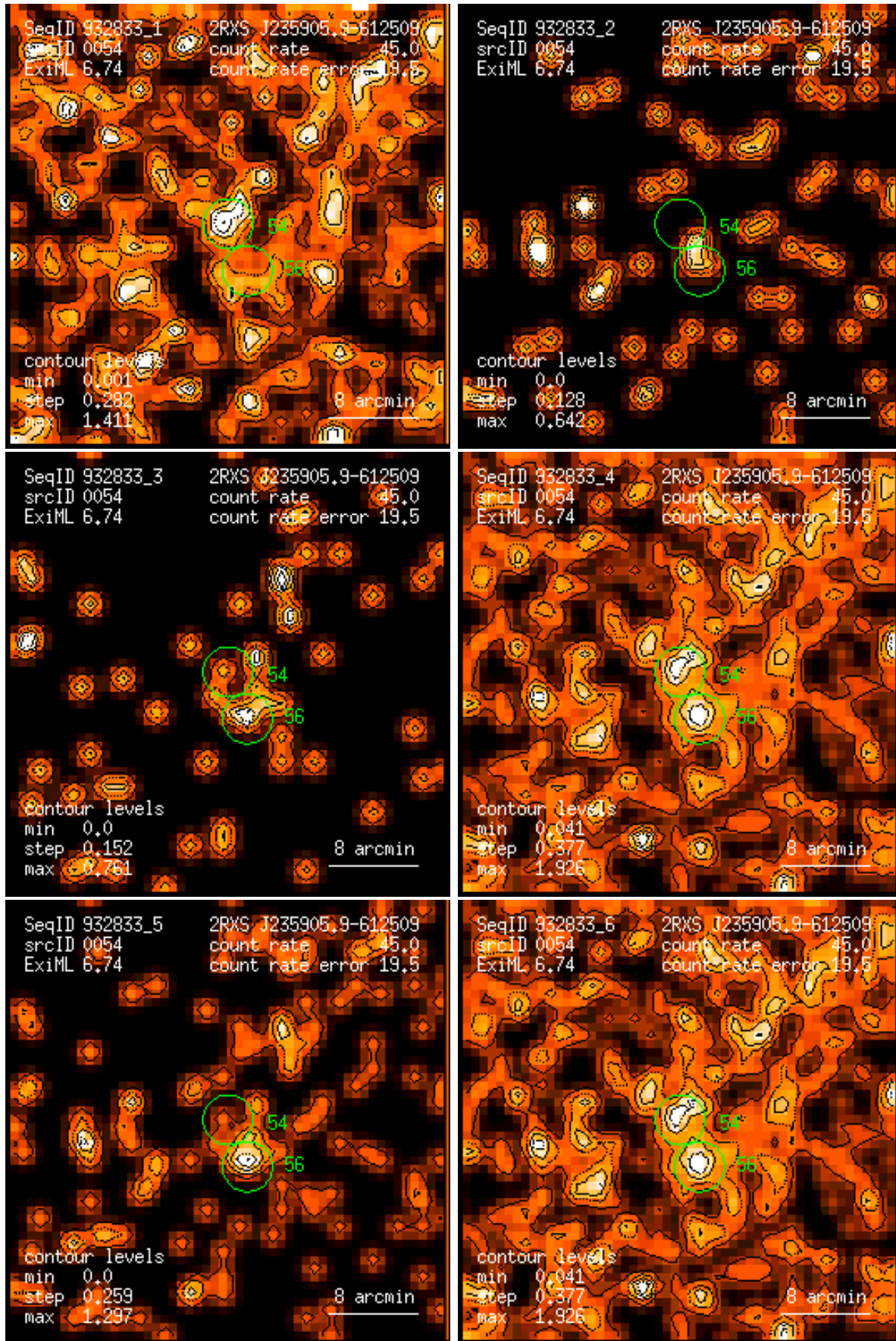
Figure 54: RASS 932833: detection 0054: band rate images, Gaussian filter: (1) PSPC channels 11 – 41, (2) 52 – 90, (3) 91 – 201, (4) 11 – 235, (5) 52 – 201, (6) 11 – 201. Broad band rates in counts/ks. Band rate contour levels in counts/ks/arcmin 2 .
