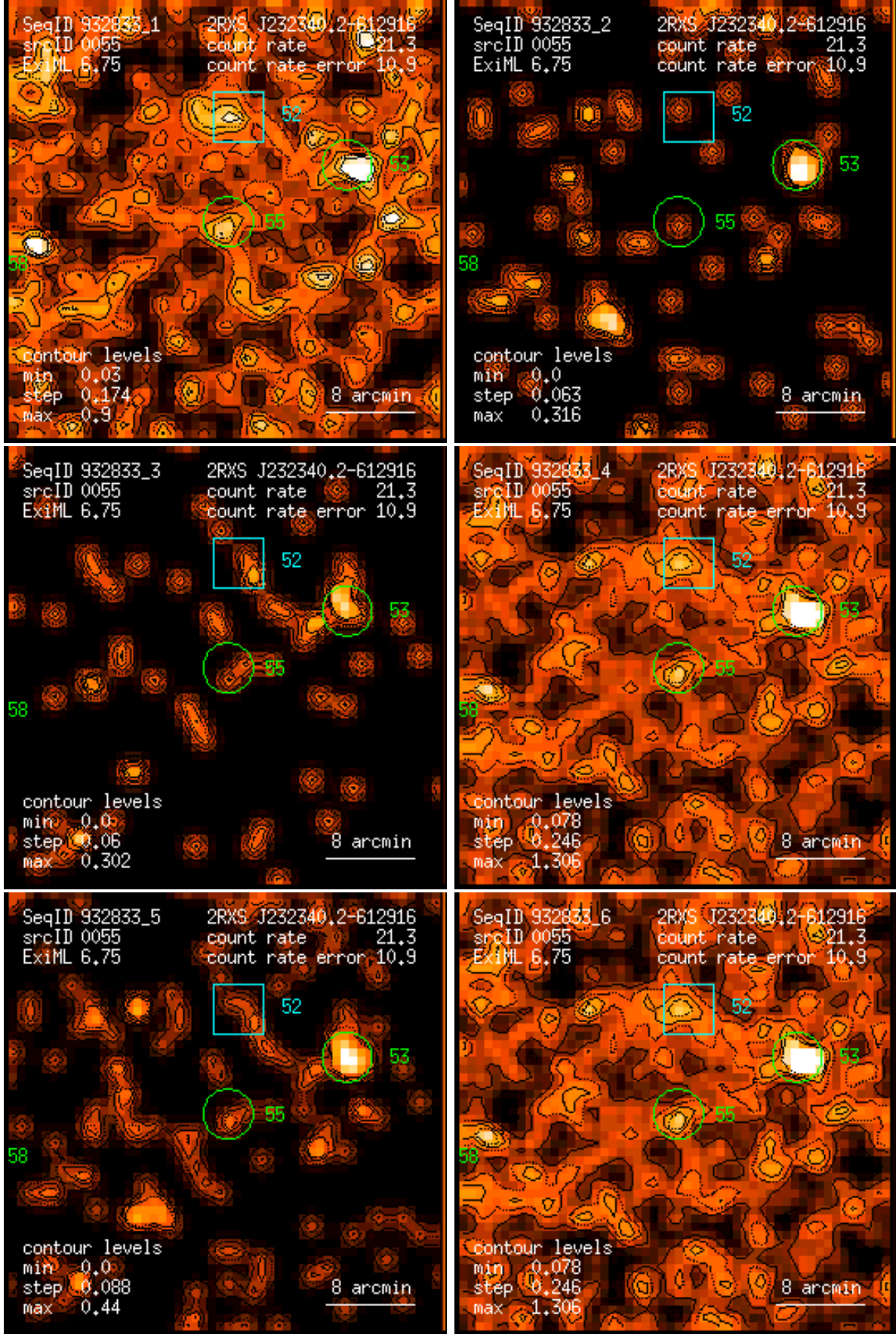
Figure 55: RASS 932833: detection 0055: band rate images, Gaussian filter: (1) PSPC channels 11 – 41, (2) 52 – 90, (3) 91 – 201, (4) 11 – 235, (5) 52 – 201, (6) 11 – 201. Broad band rates in counts/ks. Band rate contour levels in counts/ks/arcmin 2 .
