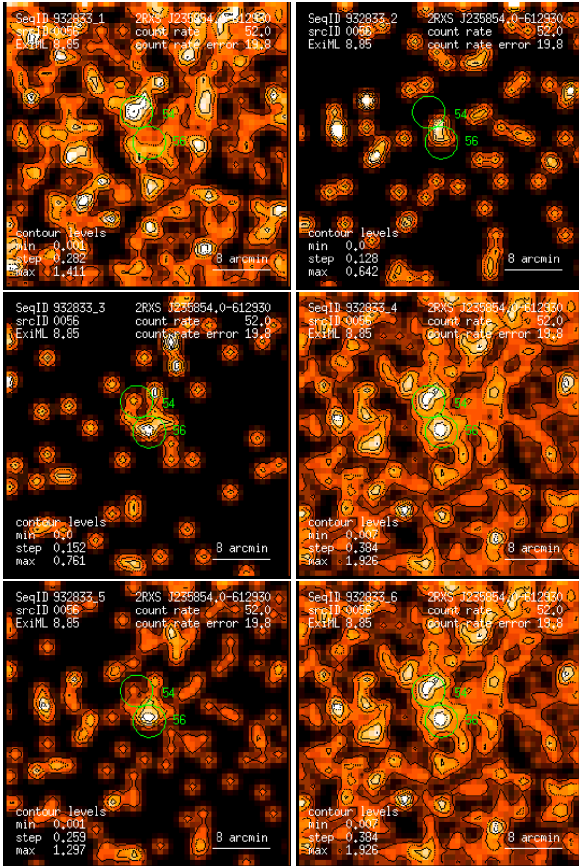
Figure 56: RASS 932833: detection 0056: band rate images, Gaussian filter: (1) PSPC channels 11 – 41, (2) 52 – 90, (3) 91 – 201, (4) 11 – 235, (5) 52 – 201, (6) 11 – 201. Broad band rates in counts/ks. Band rate contour levels in counts/ks/arcmin 2 .
