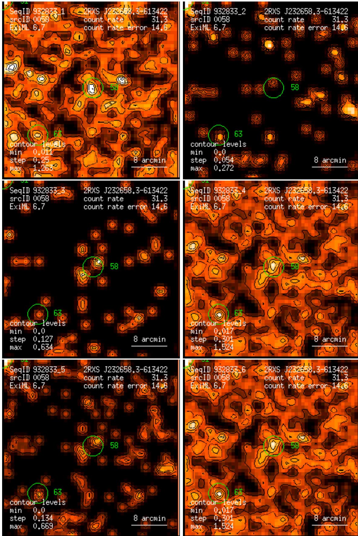
Figure 58: RASS 932833: detection 0058: band rate images, Gaussian filter: (1) PSPC channels 11 – 41, (2) 52 – 90, (3) 91 – 201, (4) 11 – 235, (5) 52 – 201, (6) 11 – 201. Broad band rates in counts/ks. Band rate contour levels in counts/ks/arcmin 2 .
