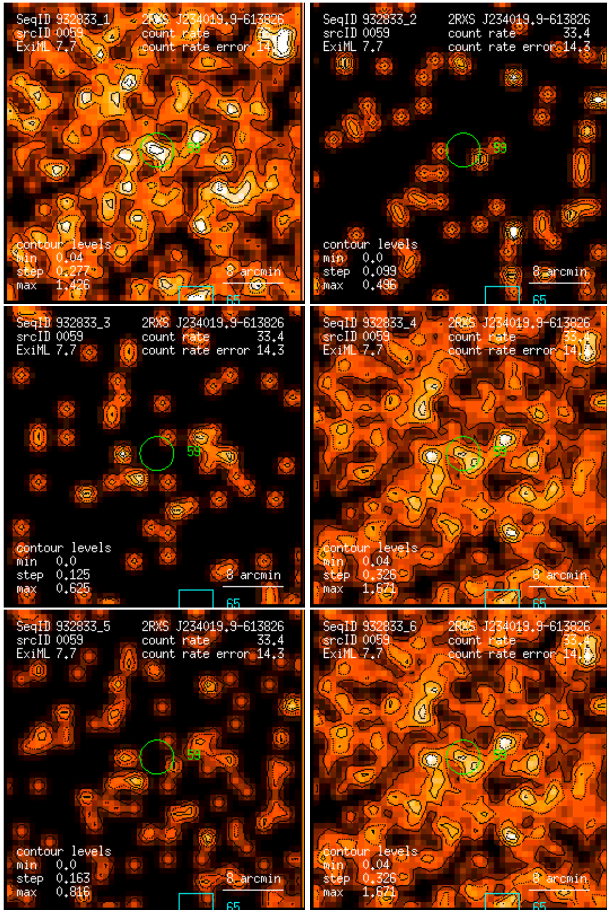
Figure 59: RASS 932833: detection 0059: band rate images, Gaussian filter: (1) PSPC channels 11 – 41, (2) 52 – 90, (3) 91 – 201, (4) 11 – 235, (5) 52 – 201, (6) 11 – 201. Broad band rates in counts/ks. Band rate contour levels in counts/ks/arcmin 2 .
