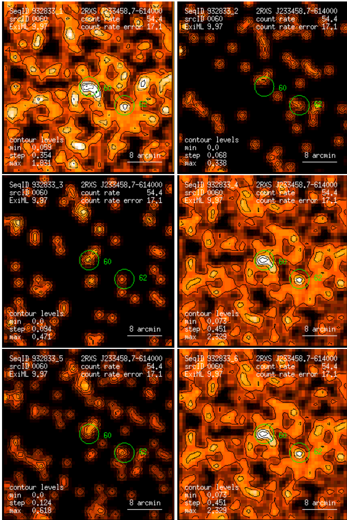
Figure 60: RASS 932833: detection 0060: band rate images, Gaussian filter: (1) PSPC channels 11 – 41, (2) 52 – 90, (3) 91 – 201, (4) 11 – 235, (5) 52 – 201, (6) 11 – 201. Broad band rates in counts/ks. Band rate contour levels in counts/ks/arcmin 2 .
