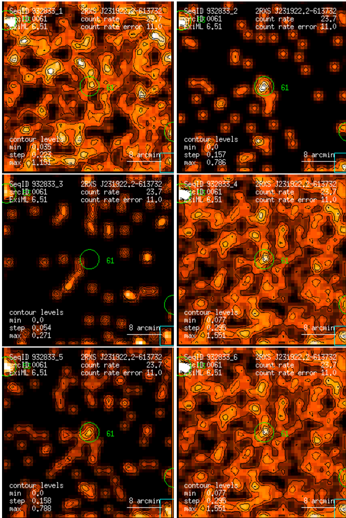
Figure 61: RASS 932833: detection 0061: band rate images, Gaussian filter: (1) PSPC channels 11 – 41, (2) 52 – 90, (3) 91 – 201, (4) 11 – 235, (5) 52 – 201, (6) 11 – 201. Broad band rates in counts/ks. Band rate contour levels in counts/ks/arcmin 2 .
