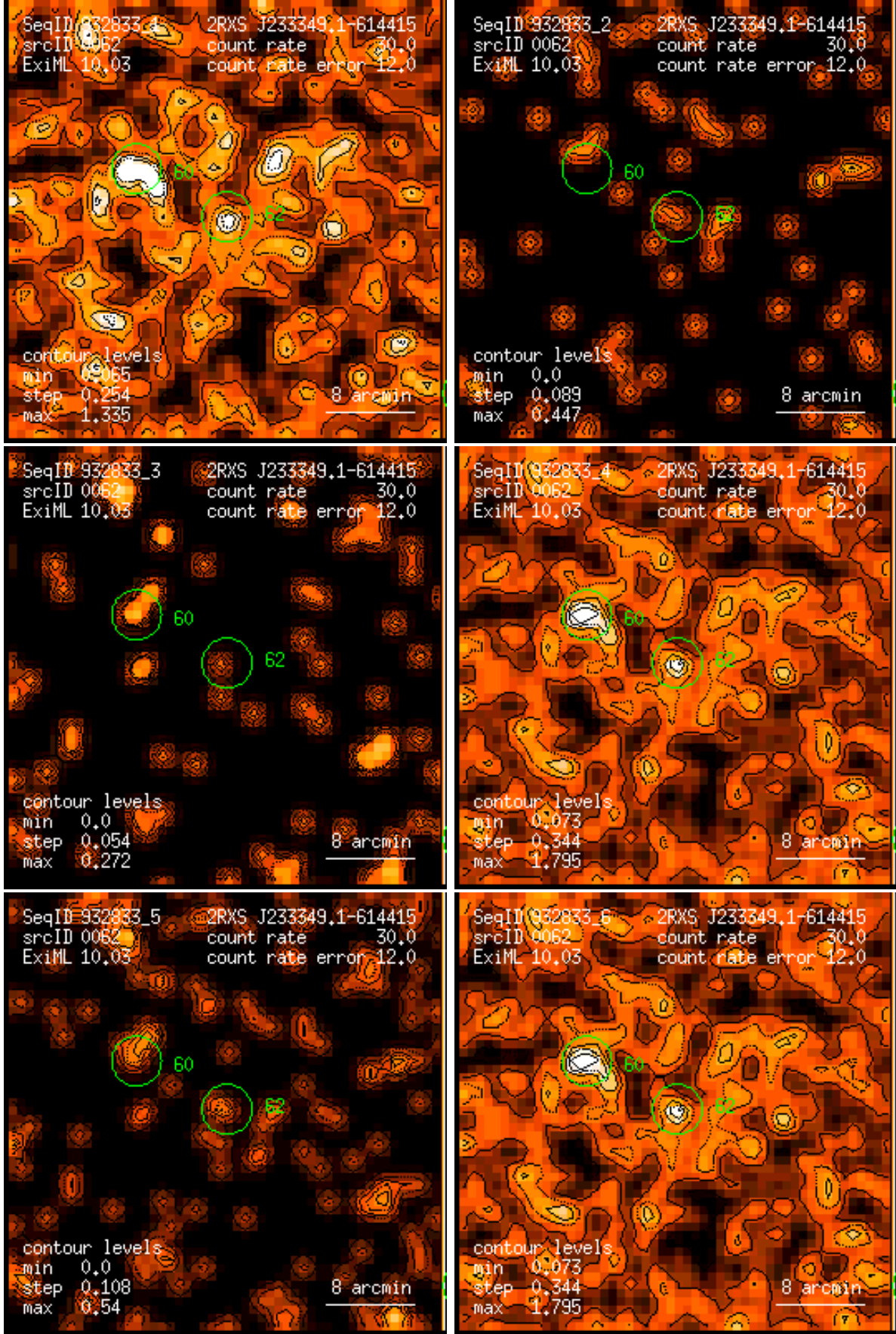
Figure 62: RASS 932833: detection 0062: band rate images, Gaussian filter: (1) PSPC channels 11 – 41, (2) 52 – 90, (3) 91 – 201, (4) 11 – 235, (5) 52 – 201, (6) 11 – 201. Broad band rates in counts/ks. Band rate contour levels in counts/ks/arcmin 2 .
