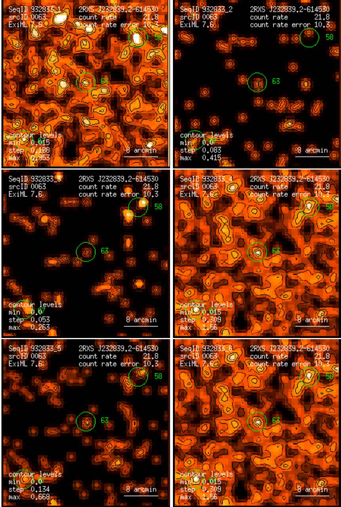
Figure 63: RASS 932833: detection 0063: band rate images, Gaussian filter: (1) PSPC channels 11 – 41, (2) 52 – 90, (3) 91 – 201, (4) 11 – 235, (5) 52 – 201, (6) 11 – 201. Broad band rates in counts/ks. Band rate contour levels in counts/ks/arcmin 2 .
