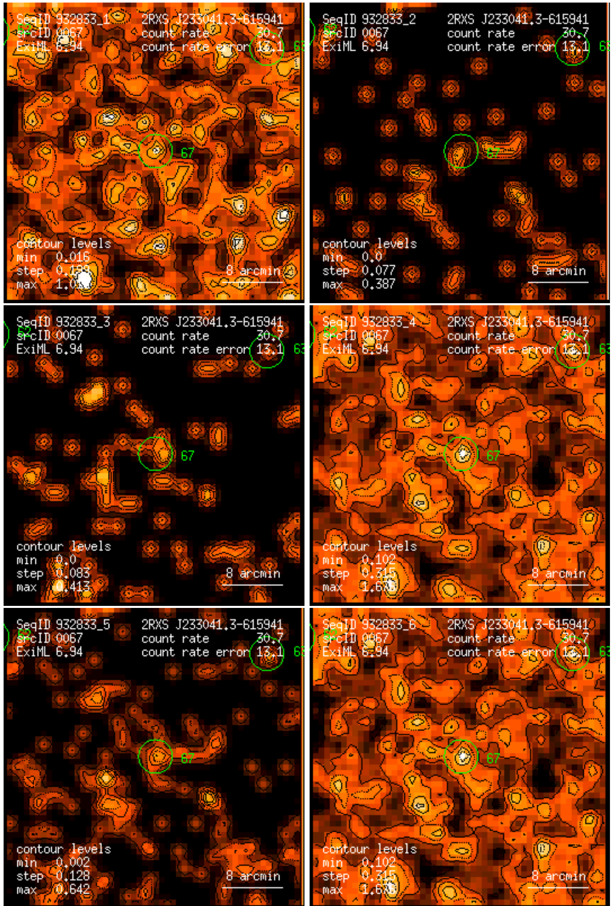
Figure 67: RASS 932833: detection 0067: band rate images, Gaussian filter: (1) PSPC channels 11 – 41, (2) 52 – 90, (3) 91 – 201, (4) 11 – 235, (5) 52 – 201, (6) 11 – 201. Broad band rates in counts/ks. Band rate contour levels in counts/ks/arcmin 2 .
