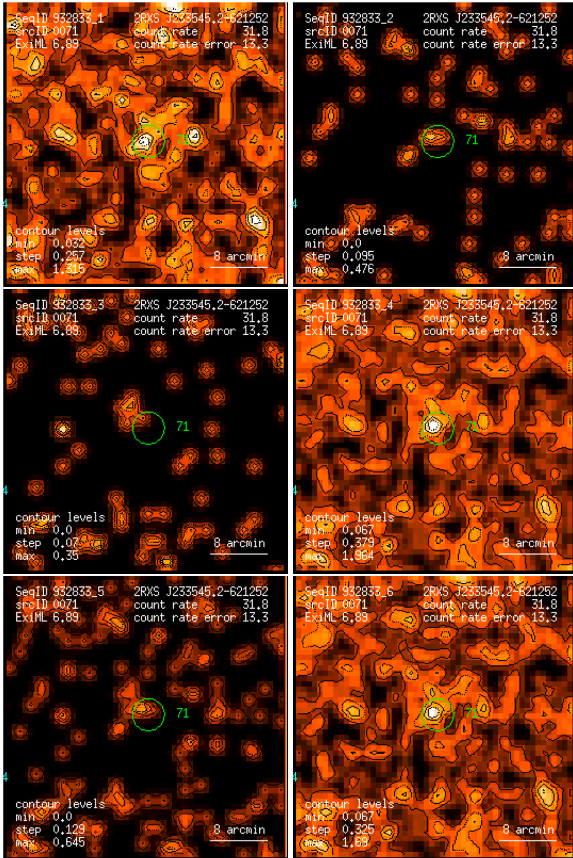
Figure 71: RASS 932833: detection 0071: band rate images, Gaussian filter: (1) PSPC channels 11 – 41, (2) 52 – 90, (3) 91 – 201, (4) 11 – 235, (5) 52 – 201, (6) 11 – 201. Broad band rates in counts/ks. Band rate contour levels in counts/ks/arcmin 2 .
