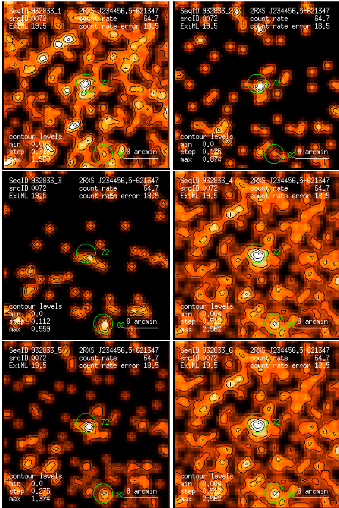
Figure 72: RASS 932833: detection 0072: band rate images, Gaussian filter: (1) PSPC channels 11 – 41, (2) 52 – 90, (3) 91 – 201, (4) 11 – 235, (5) 52 – 201, (6) 11 – 201. Broad band rates in counts/ks. Band rate contour levels in counts/ks/arcmin 2 .
