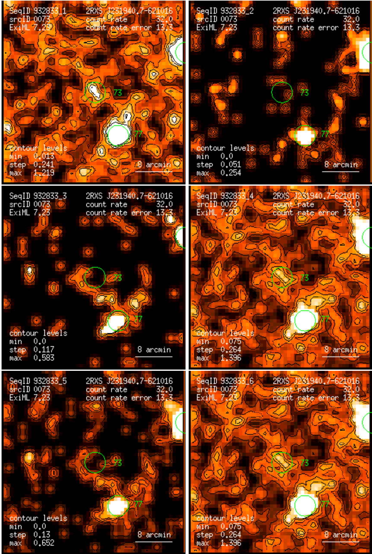
Figure 73: RASS 932833: detection 0073: band rate images, Gaussian filter: (1) PSPC channels 11 – 41, (2) 52 – 90, (3) 91 – 201, (4) 11 – 235, (5) 52 – 201, (6) 11 – 201. Broad band rates in counts/ks. Band rate contour levels in counts/ks/arcmin 2 .
