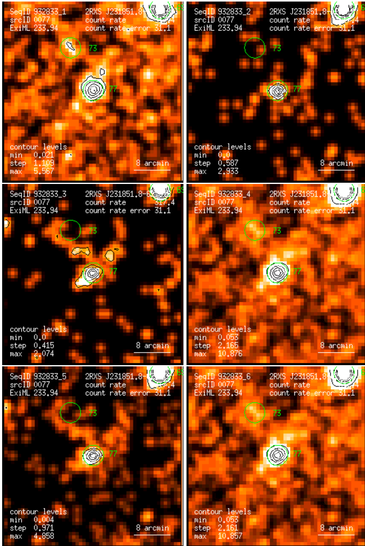
Figure 77: RASS 932833: detection 0077: band rate images, Gaussian filter: (1) PSPC channels 11 – 41, (2) 52 – 90, (3) 91 – 201, (4) 11 – 235, (5) 52 – 201, (6) 11 – 201. Broad band rates in counts/ks. Band rate contour levels in counts/ks/arcmin 2 .
