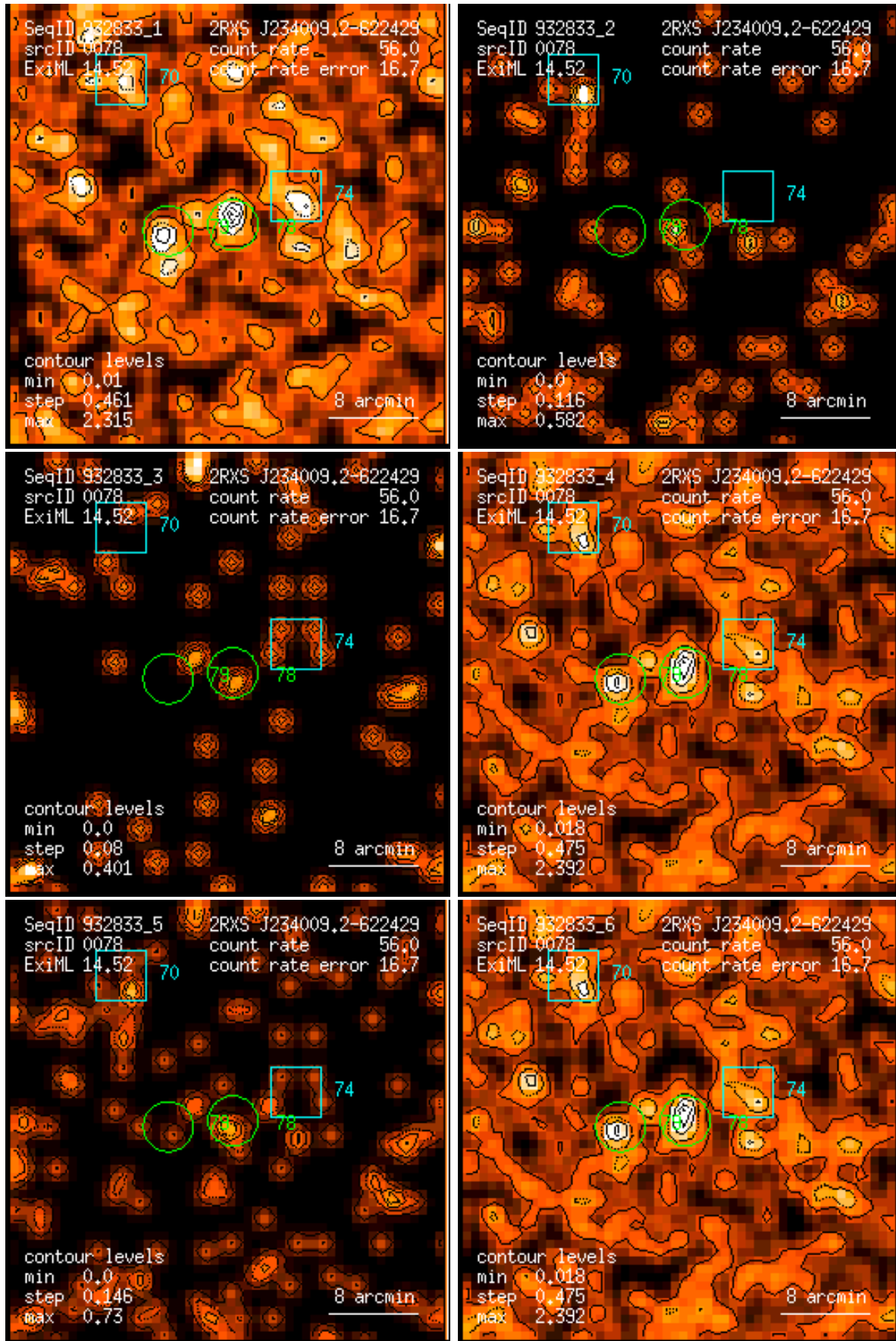
Figure 78: RASS 932833: detection 0078: band rate images, Gaussian filter: (1) PSPC channels 11 – 41, (2) 52 – 90, (3) 91 – 201, (4) 11 – 235, (5) 52 – 201, (6) 11 – 201. Broad band rates in counts/ks. Band rate contour levels in counts/ks/arcmin 2 .
