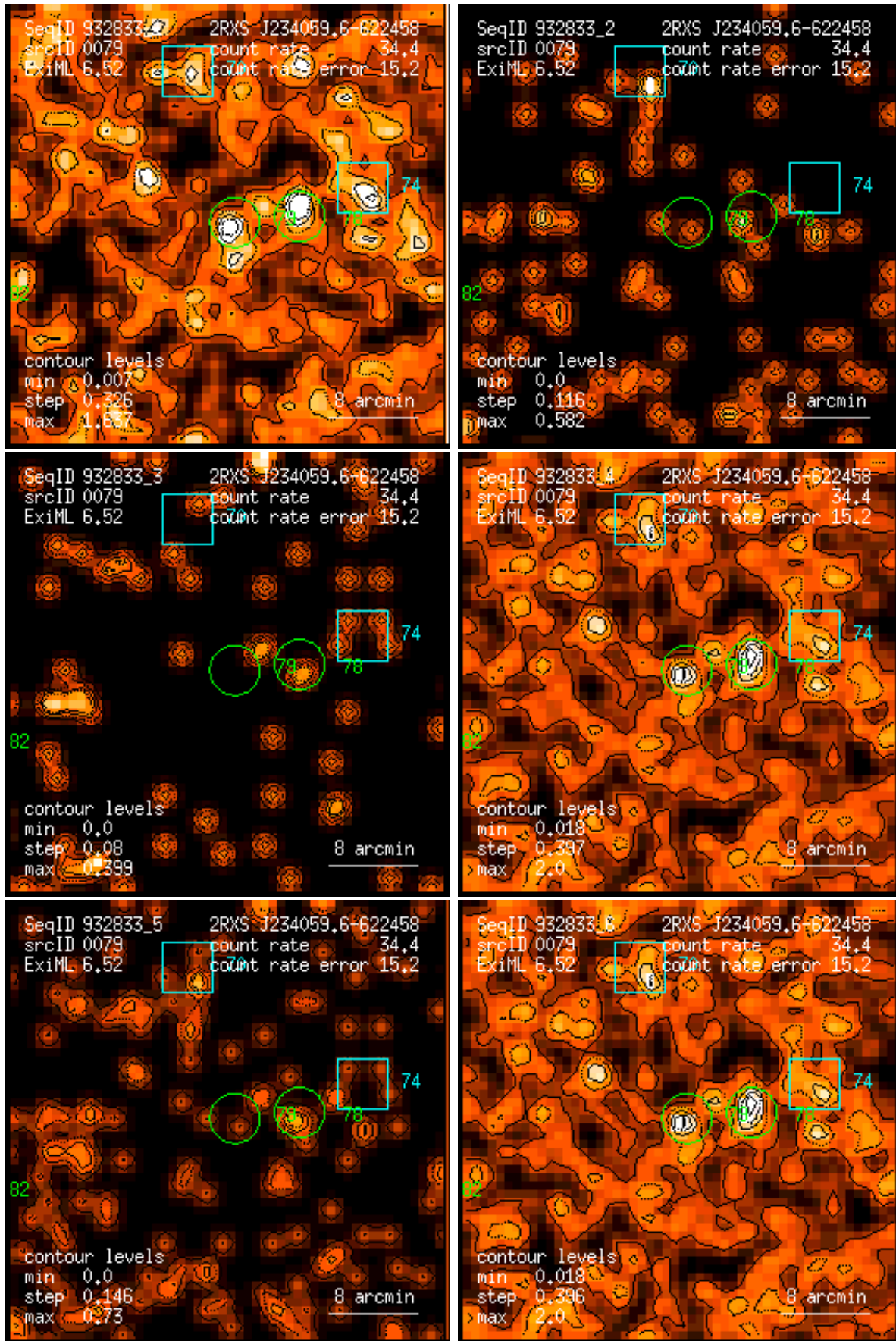
Figure 79: RASS 932833: detection 0079: band rate images, Gaussian filter: (1) PSPC channels 11 – 41, (2) 52 – 90, (3) 91 – 201, (4) 11 – 235, (5) 52 – 201, (6) 11 – 201. Broad band rates in counts/ks. Band rate contour levels in counts/ks/arcmin 2 .
