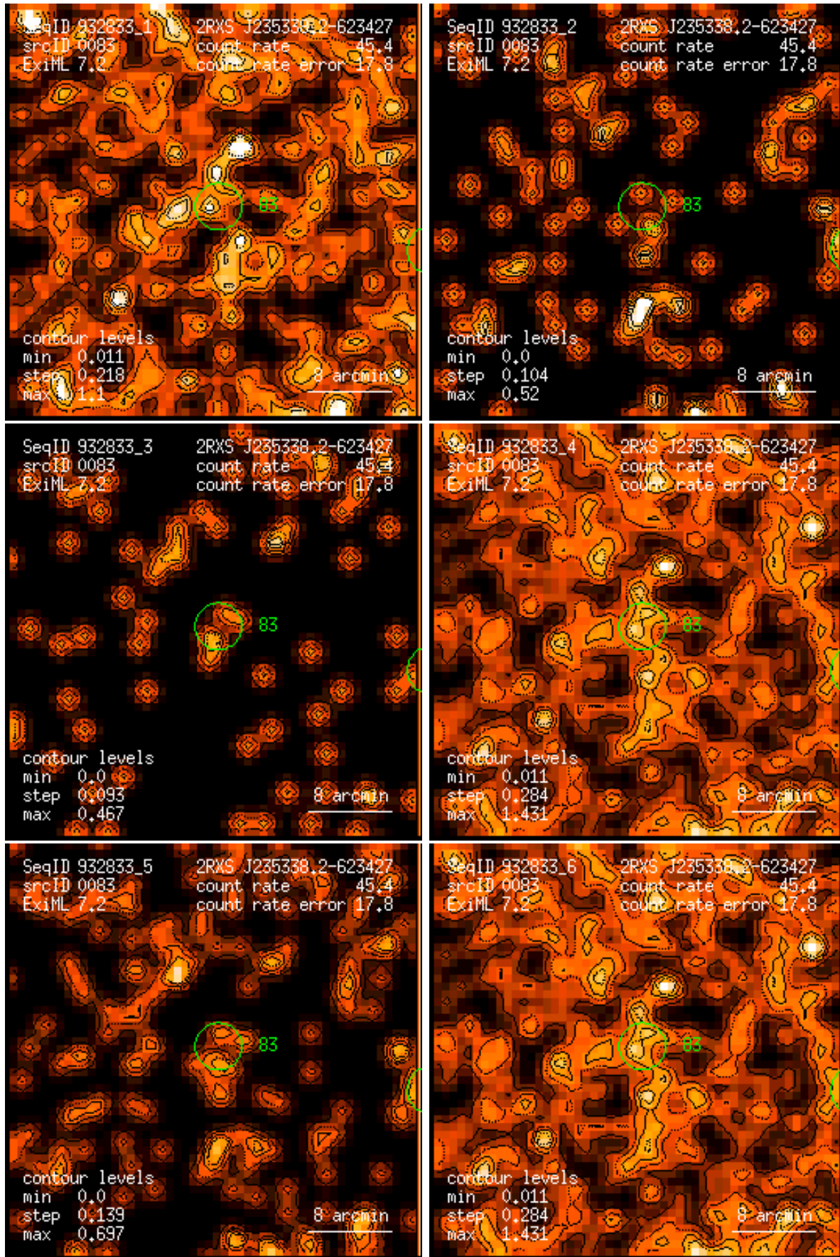
Figure 83: RASS 932833: detection 0083: band rate images, Gaussian filter: (1) PSPC channels 11 – 41, (2) 52 – 90, (3) 91 – 201, (4) 11 – 235, (5) 52 – 201, (6) 11 – 201. Broad band rates in counts/ks. Band rate contour levels in counts/ks/arcmin 2 .
