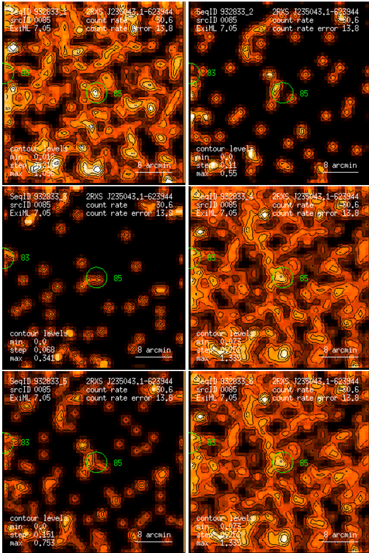
Figure 85: RASS 932833: detection 0085: band rate images, Gaussian filter: (1) PSPC channels 11 – 41, (2) 52 – 90, (3) 91 – 201, (4) 11 – 235, (5) 52 – 201, (6) 11 – 201. Broad band rates in counts/ks. Band rate contour levels in counts/ks/arcmin 2 .
