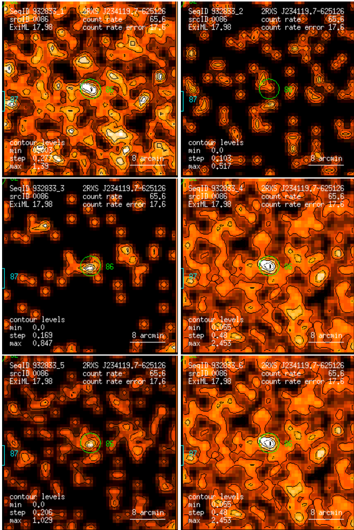
Figure 86: RASS 932833: detection 0086: band rate images, Gaussian filter: (1) PSPC channels 11 – 41, (2) 52 – 90, (3) 91 – 201, (4) 11 – 235, (5) 52 – 201, (6) 11 – 201. Broad band rates in counts/ks. Band rate contour levels in counts/ks/arcmin 2 .
