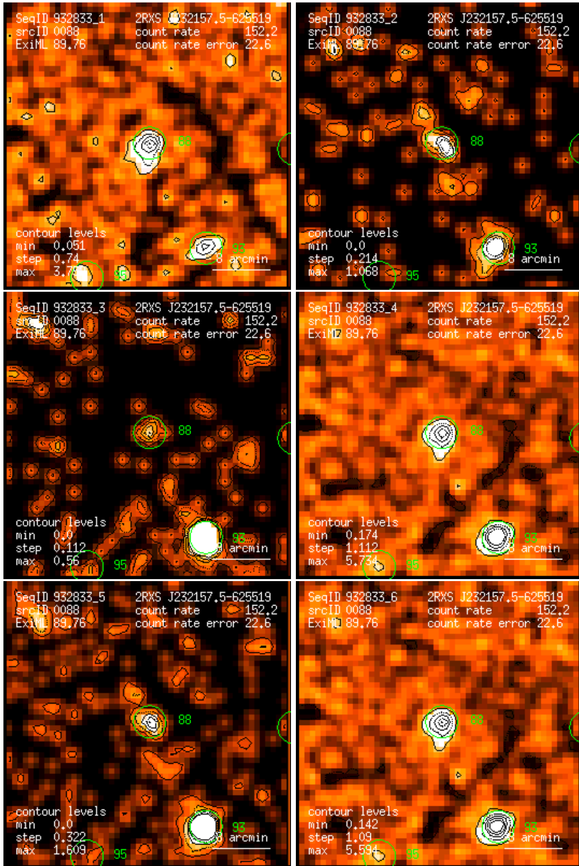
Figure 88: RASS 932833: detection 0088: band rate images, Gaussian filter: (1) PSPC channels 11 – 41, (2) 52 – 90, (3) 91 – 201, (4) 11 – 235, (5) 52 – 201, (6) 11 – 201. Broad band rates in counts/ks. Band rate contour levels in counts/ks/arcmin 2 .
