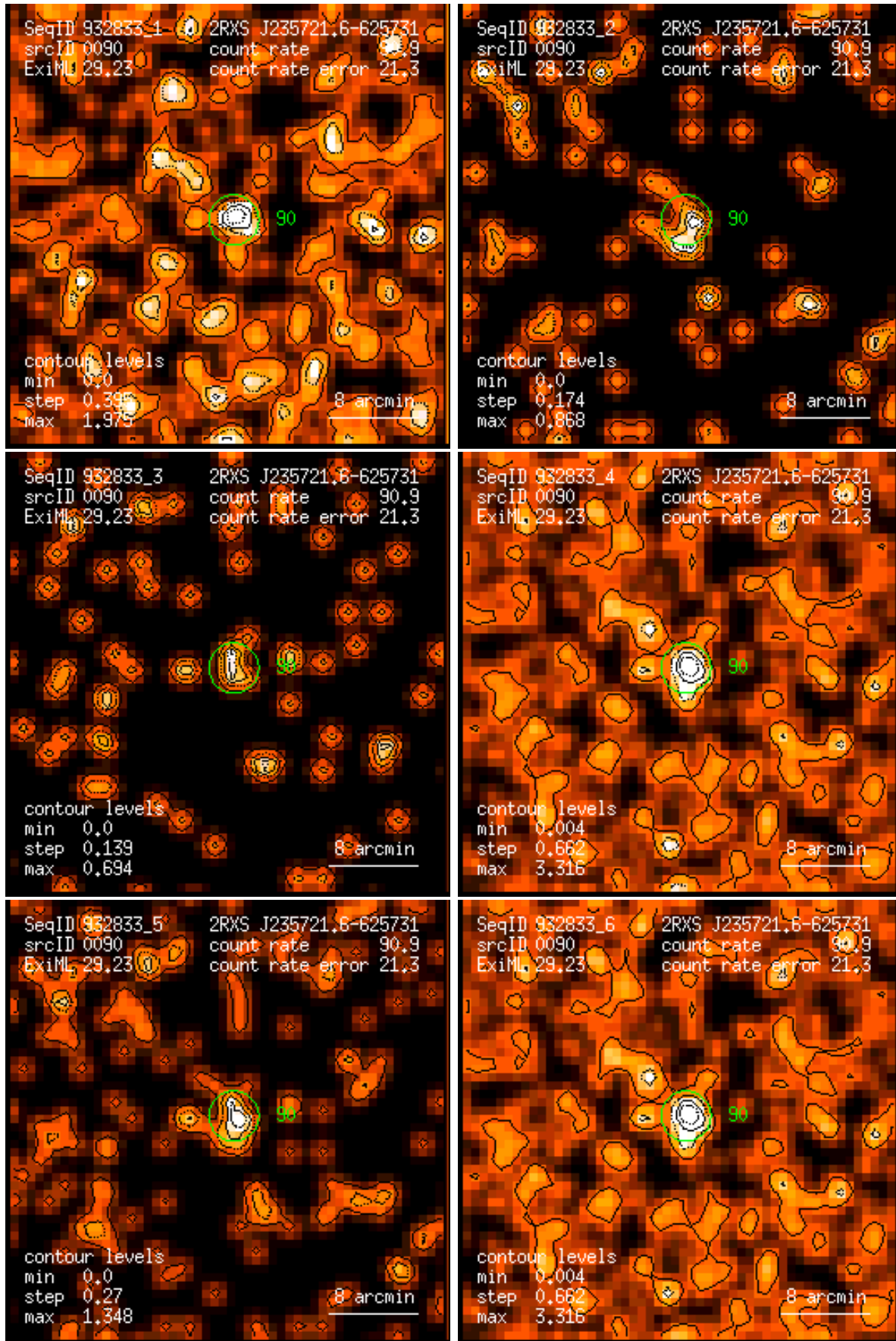
Figure 90: RASS 932833: detection 0090: band rate images, Gaussian filter: (1) PSPC channels 11 – 41, (2) 52 – 90, (3) 91 – 201, (4) 11 – 235, (5) 52 – 201, (6) 11 – 201. Broad band rates in counts/ks. Band rate contour levels in counts/ks/arcmin 2 .
