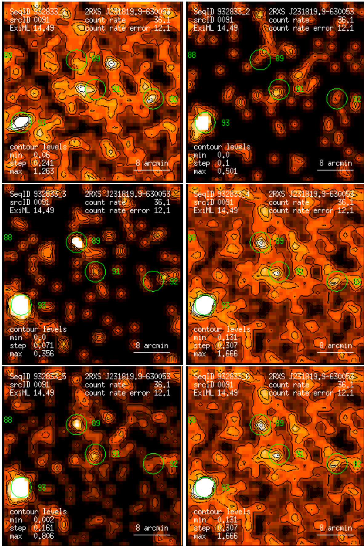
Figure 91: RASS 932833: detection 0091: band rate images, Gaussian filter: (1) PSPC channels 11 – 41, (2) 52 – 90, (3) 91 – 201, (4) 11 – 235, (5) 52 – 201, (6) 11 – 201. Broad band rates in counts/ks. Band rate contour levels in counts/ks/arcmin 2 .
