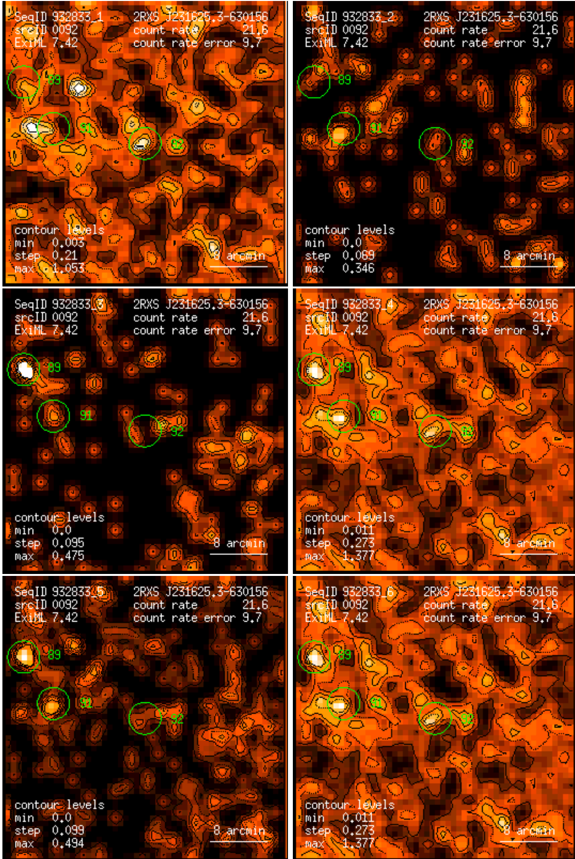
Figure 92: RASS 932833: detection 0092: band rate images, Gaussian filter: (1) PSPC channels 11 – 41, (2) 52 – 90, (3) 91 – 201, (4) 11 – 235, (5) 52 – 201, (6) 11 – 201. Broad band rates in counts/ks. Band rate contour levels in counts/ks/arcmin 2 .
