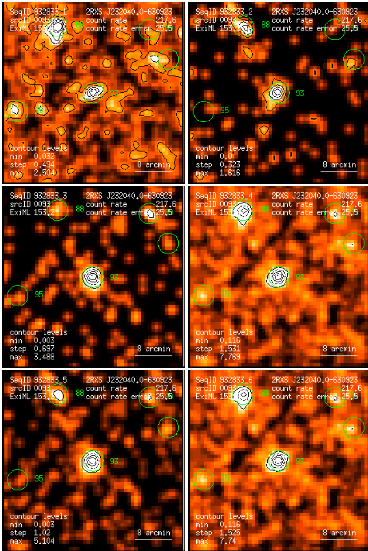
Figure 93: RASS 932833: detection 0093: band rate images, Gaussian filter: (1) PSPC channels 11 – 41, (2) 52 – 90, (3) 91 – 201, (4) 11 – 235, (5) 52 – 201, (6) 11 – 201. Broad band rates in counts/ks. Band rate contour levels in counts/ks/arcmin 2 .
