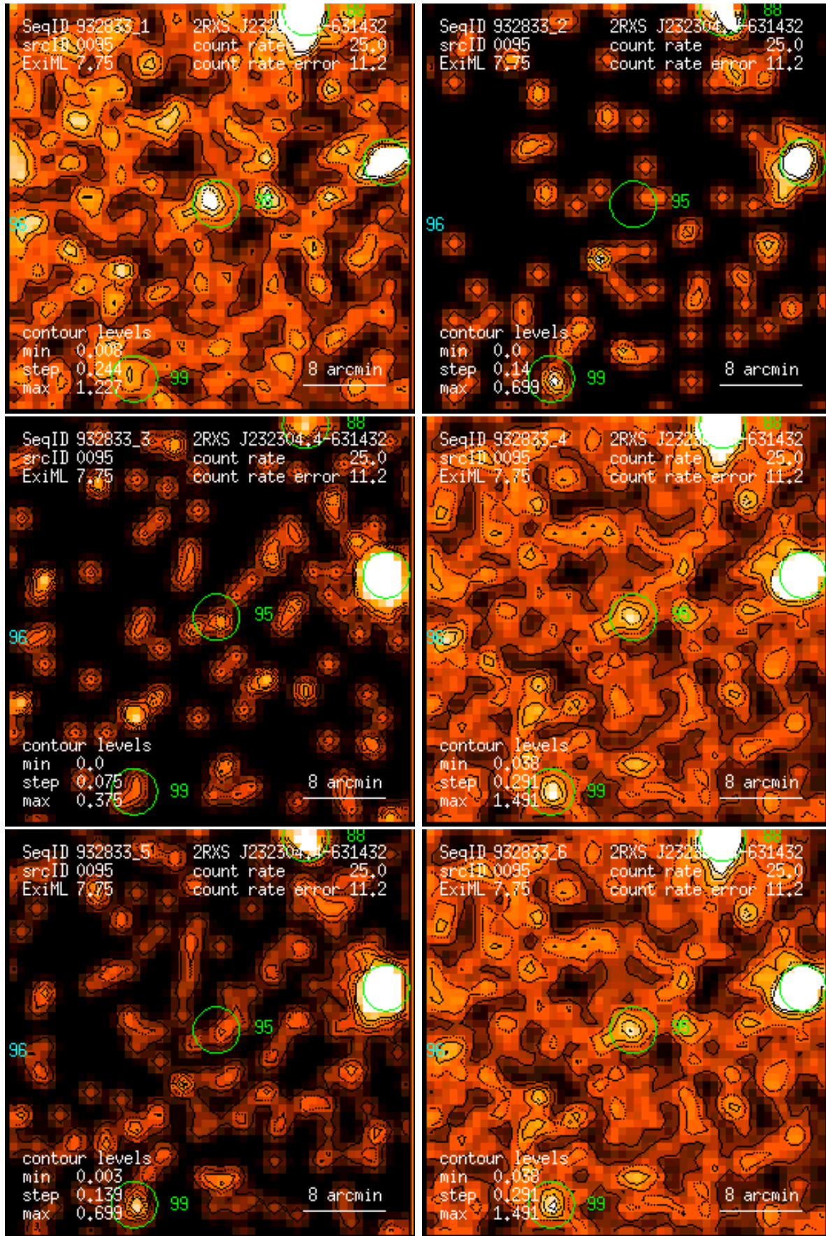
Figure 95: RASS 932833: detection 0095: band rate images, Gaussian filter: (1) PSPC channels 11 – 41, (2) 52 – 90, (3) 91 – 201, (4) 11 – 235, (5) 52 – 201, (6) 11 – 201. Broad band rates in counts/ks. Band rate contour levels in counts/ks/arcmin 2 .
