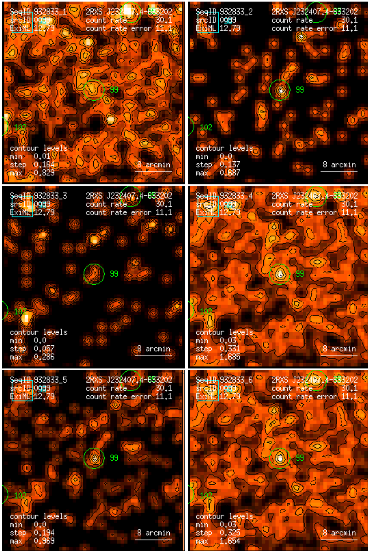
Figure 99: RASS 932833: detection 0099: band rate images, Gaussian filter: (1) PSPC channels 11 – 41, (2) 52 – 90, (3) 91 – 201, (4) 11 – 235, (5) 52 – 201, (6) 11 – 201. Broad band rates in counts/ks. Band rate contour levels in counts/ks/arcmin 2 .
