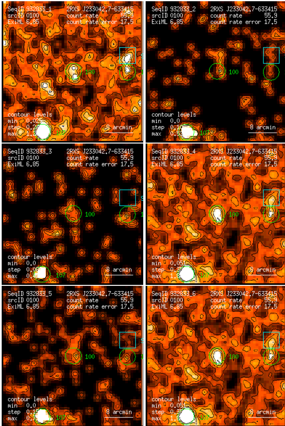
Figure 100: RASS 932833: detection 0100: band rate images, Gaussian filter: (1) PSPC channels 11 – 41, (2) 52 – 90, (3) 91 – 201, (4) 11 – 235, (5) 52 – 201, (6) 11 – 201. Broad band rates in counts/ks. Band rate contour levels in counts/ks/arcmin 2 .
