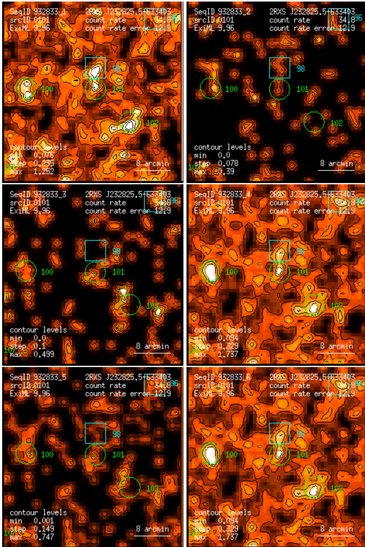
Figure 101: RASS 932833: detection 0101: band rate images, Gaussian filter: (1) PSPC channels 11 – 41, (2) 52 – 90, (3) 91 – 201, (4) 11 – 235, (5) 52 – 201, (6) 11 – 201. Broad band rates in counts/ks. Band rate contour levels in counts/ks/arcmin 2 .
