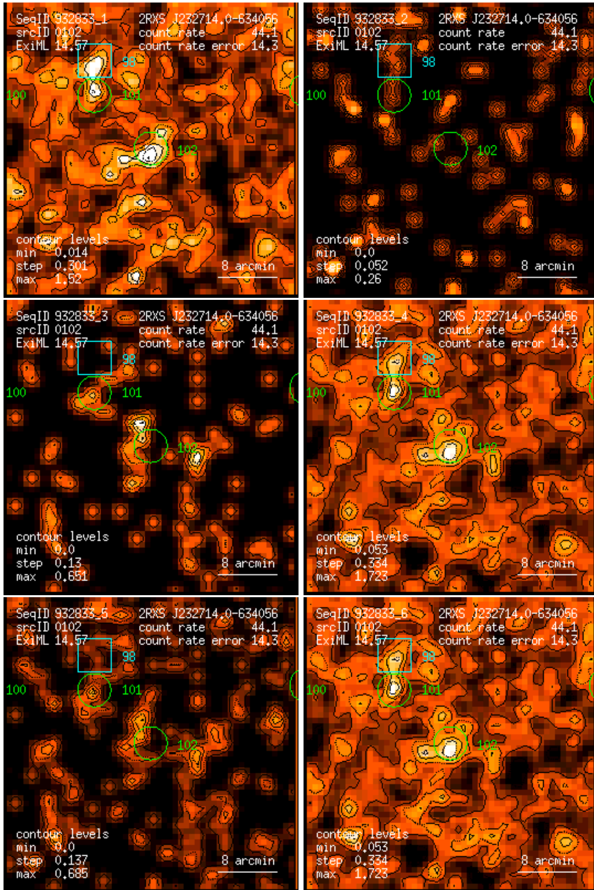
Figure 102: RASS 932833: detection 0102: band rate images, Gaussian filter: (1) PSPC channels 11 – 41, (2) 52 – 90, (3) 91 – 201, (4) 11 – 235, (5) 52 – 201, (6) 11 – 201. Broad band rates in counts/ks. Band rate contour levels in counts/ks/arcmin 2 .
