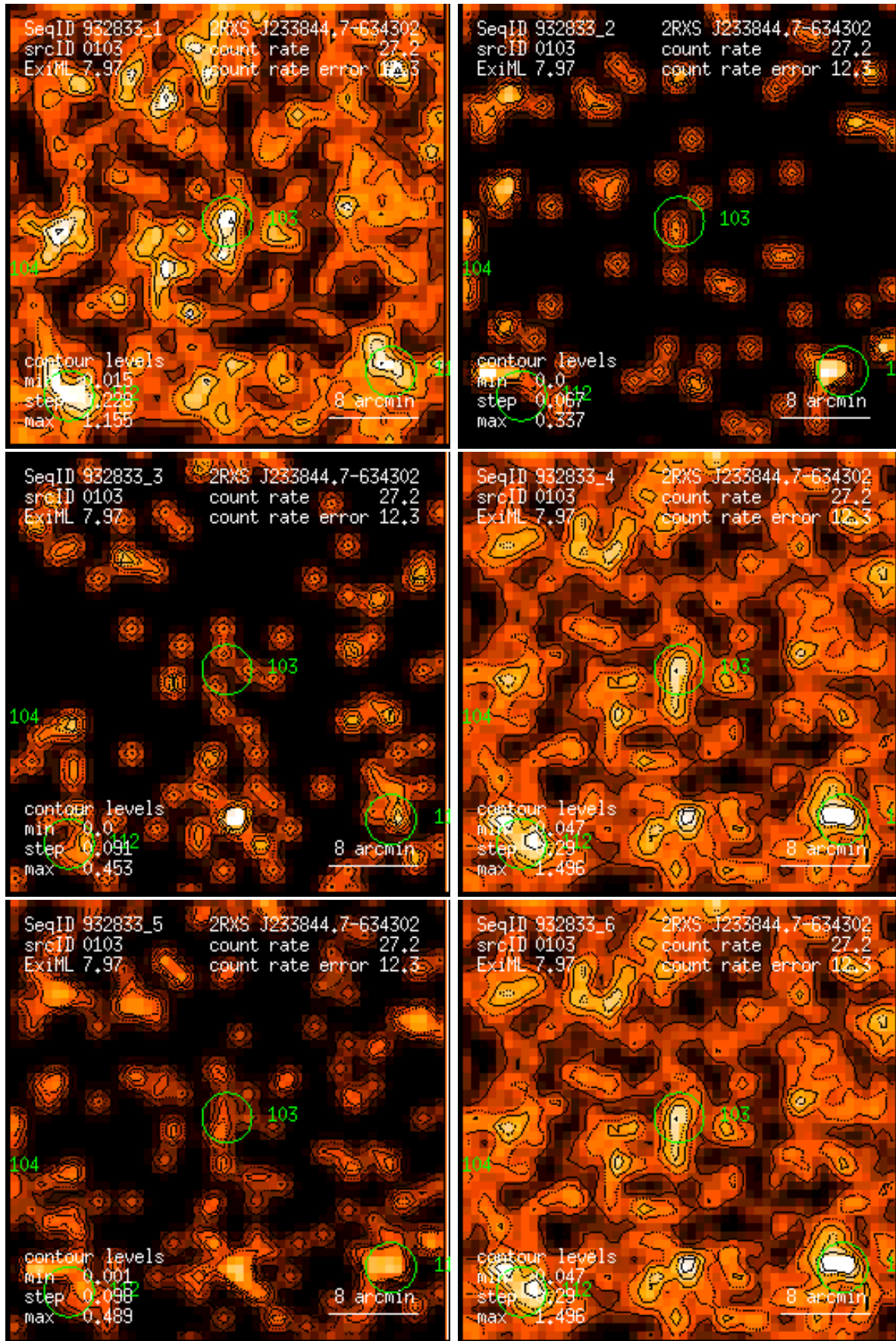
Figure 103: RASS 932833: detection 0103: band rate images, Gaussian filter: (1) PSPC channels 11 – 41, (2) 52 – 90, (3) 91 – 201, (4) 11 – 235, (5) 52 – 201, (6) 11 – 201. Broad band rates in counts/ks. Band rate contour levels in counts/ks/arcmin 2 .
