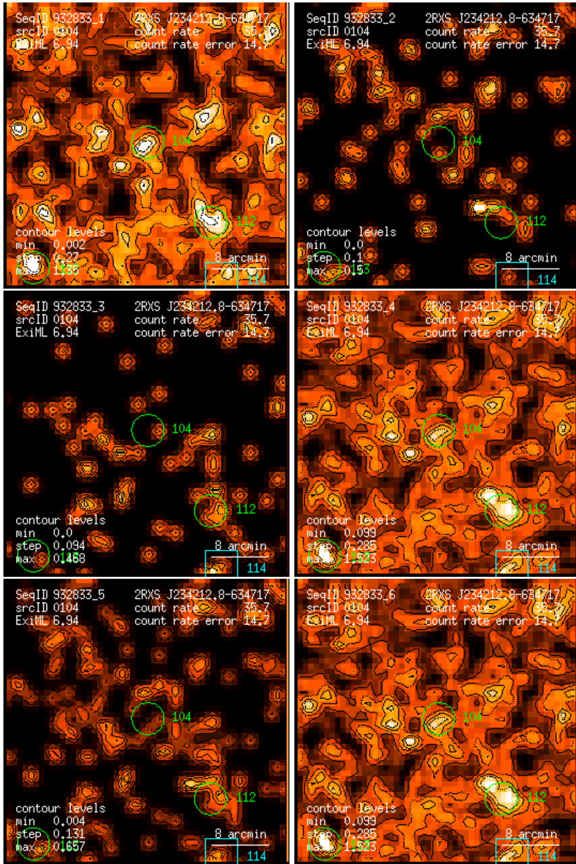
Figure 104: RASS 932833: detection 0104: band rate images, Gaussian filter: (1) PSPC channels 11 – 41, (2) 52 – 90, (3) 91 – 201, (4) 11 – 235, (5) 52 – 201, (6) 11 – 201. Broad band rates in counts/ks. Band rate contour levels in counts/ks/arcmin 2 .
