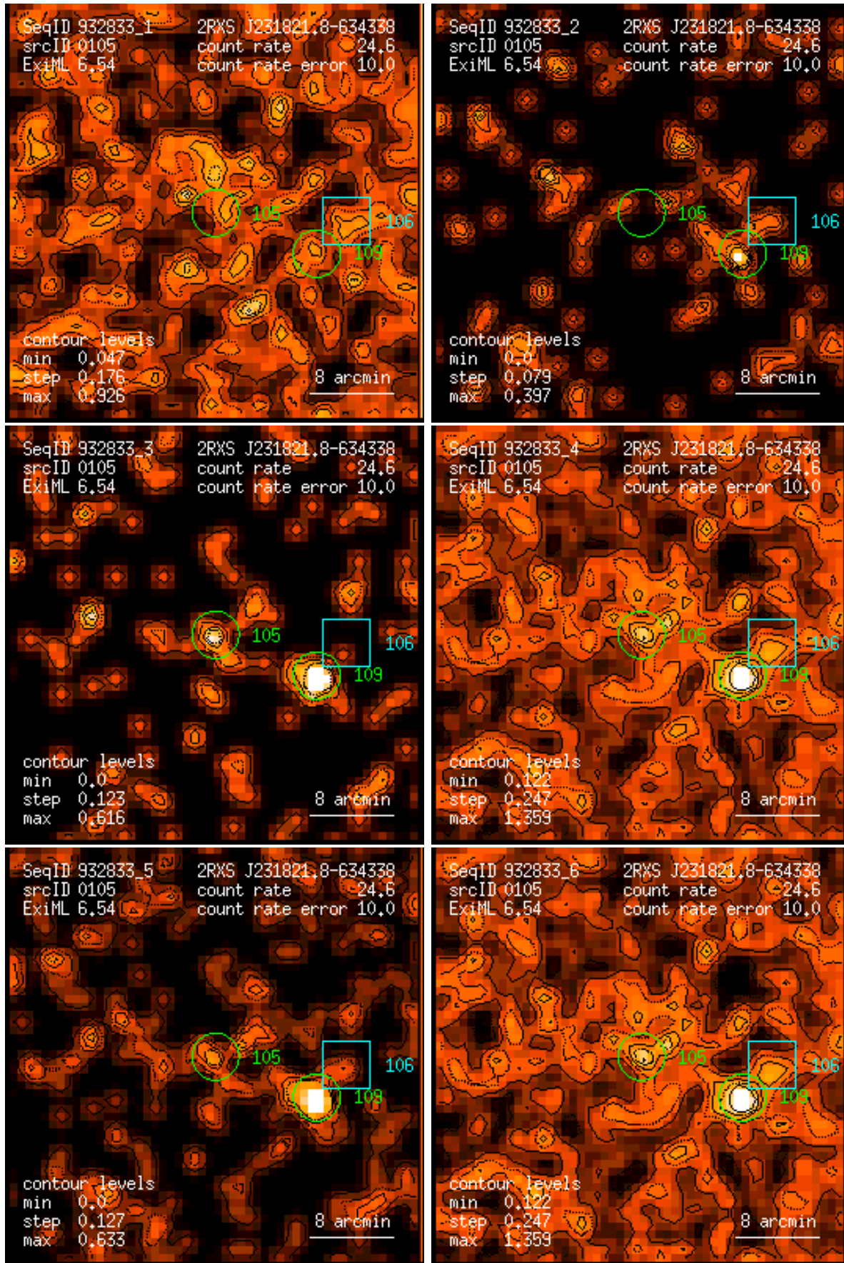
Figure 105: RASS 932833: detection 0105: band rate images, Gaussian filter: (1) PSPC channels 11 – 41, (2) 52 – 90, (3) 91 – 201, (4) 11 – 235, (5) 52 – 201, (6) 11 – 201. Broad band rates in counts/ks. Band rate contour levels in counts/ks/arcmin 2 .
