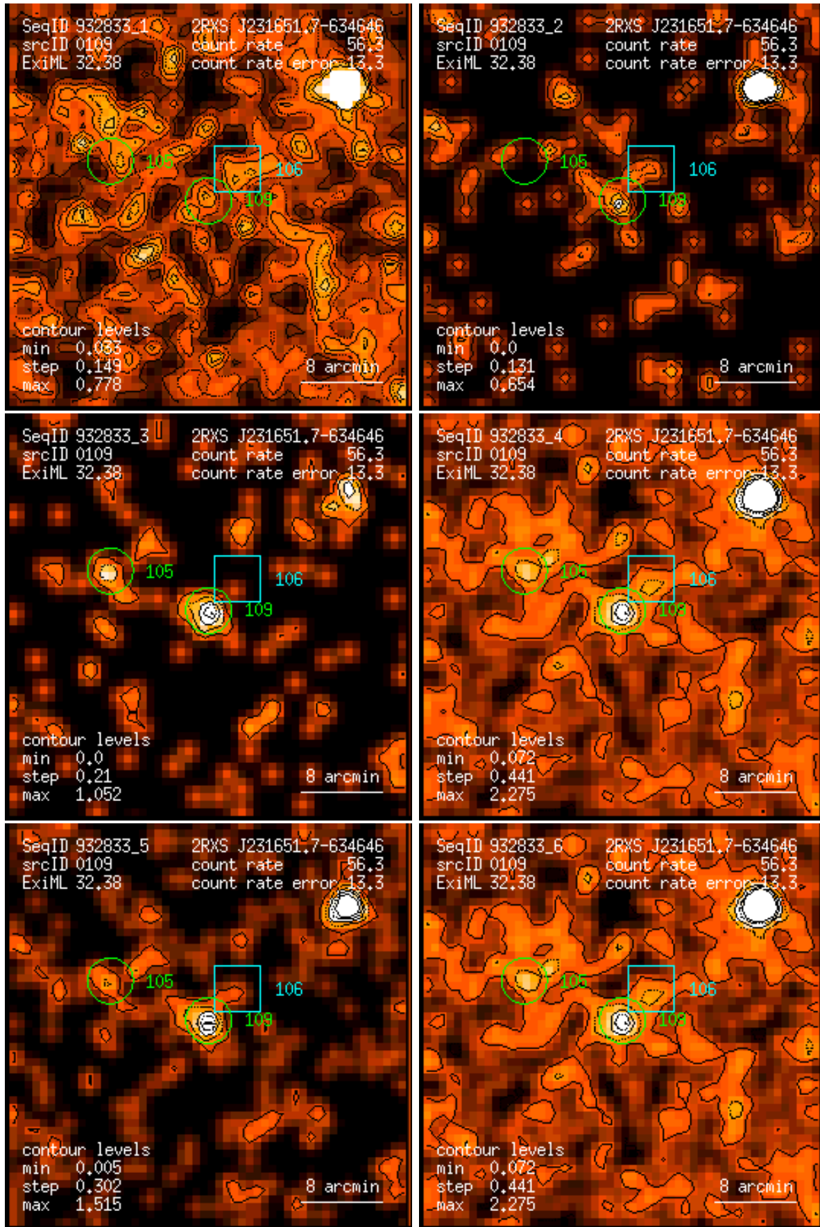
Figure 109: RASS 932833: detection 0109: band rate images, Gaussian filter: (1) PSPC channels 11 – 41, (2) 52 – 90, (3) 91 – 201, (4) 11 – 235, (5) 52 – 201, (6) 11 – 201. Broad band rates in counts/ks. Band rate contour levels in counts/ks/arcmin 2 .
