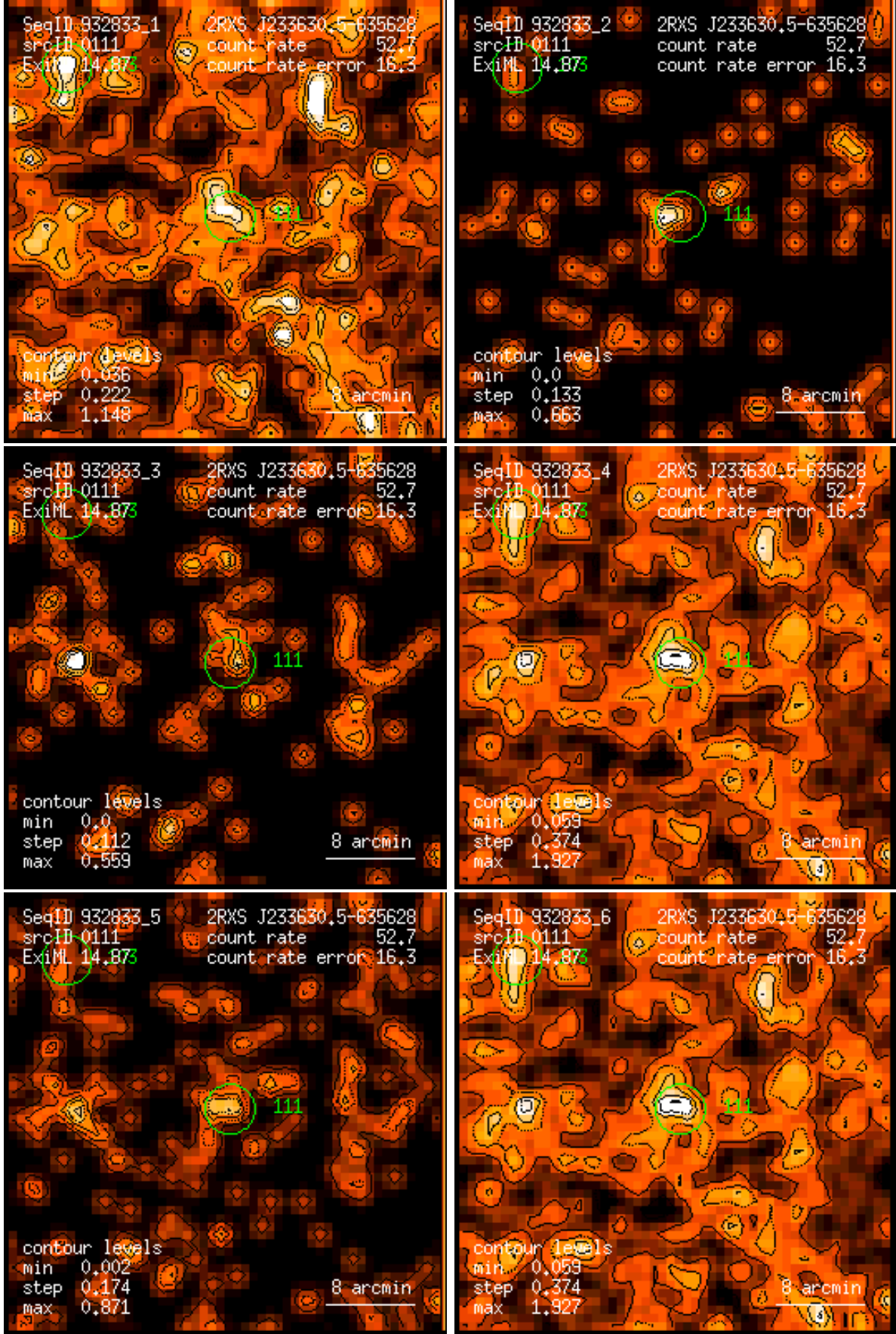
Figure 111: RASS 932833: detection 0111: band rate images, Gaussian filter: (1) PSPC channels 11 – 41, (2) 52 – 90, (3) 91 – 201, (4) 11 – 235, (5) 52 – 201, (6) 11 – 201. Broad band rates in counts/ks. Band rate contour levels in counts/ks/arcmin 2 .
